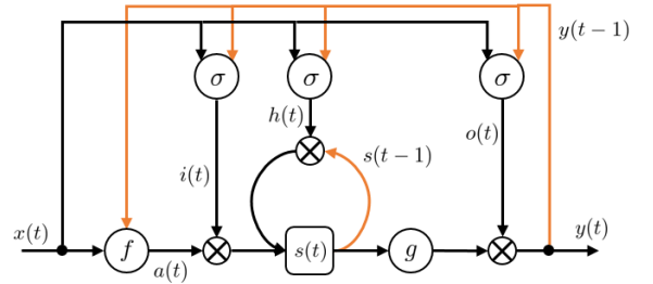
Fig. 2. Example of LSTM neurons in a hidden layer and description of the inner architecture of cells. Orange arrows show data from previous step.
