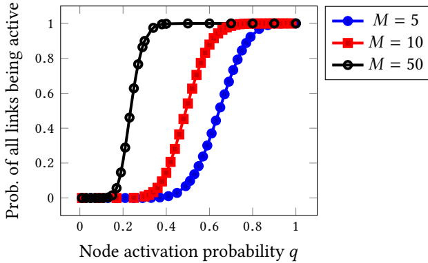
Fig. 9. Probability that all links are active in the star shaped network in Figure 8 as a function of the node activation probability q .
