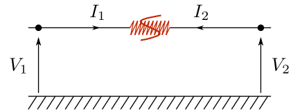
Fig. 2. Symbol for the linearized diode
