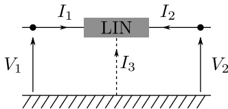
Fig. 4. Symbol for transmission lines
