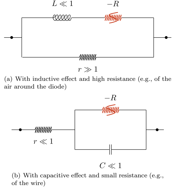
Fig. 15. Two realistic models of a linearized diode
