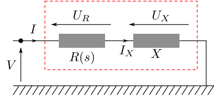
Fig. 11. Composition of a grounded branch and a dipole in series
