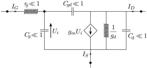
Fig. 16. Intrinsic model of a linearized transistor
