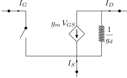
Fig. 6. Model for the linearized controlled current source.
