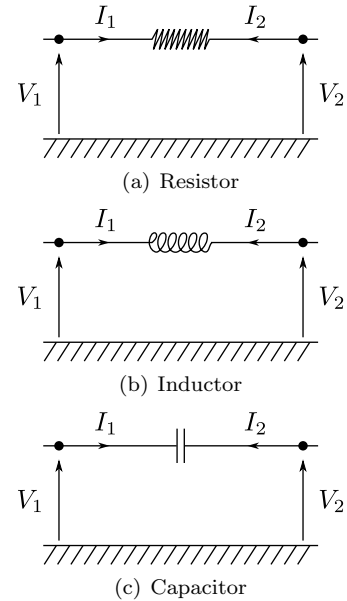
Fig. 1. Symbols for linear dipoles
