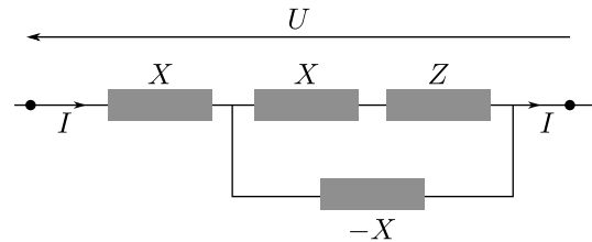
Fig. 12. The inverter network
