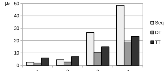
Fig. 7. ROSACE: (1) Communication only, (2) ROSACE+0, (3) ROSACE+100 and (4) ROSACE+200 cycles in each node are compared for Sequential, Data-Triggered and Time-Triggered methods.
