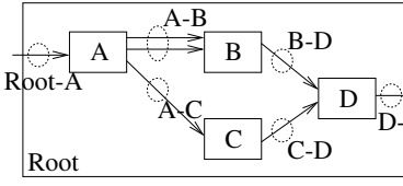
Fig. 2. Extraction of channels from a program.
