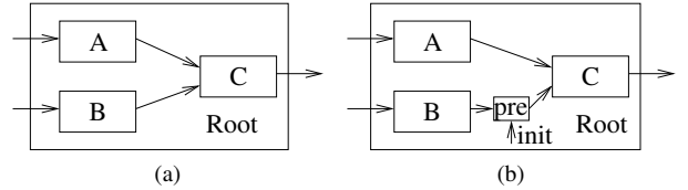
Fig. 1. Synchronous Data-Flow Networks. (a) A and B can be computed in parallel and B and C must be in sequence. (b) B can be computed in parallel with both A and C because of the delay ( pre ).
