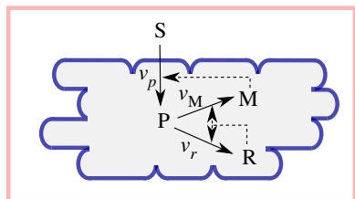
Figure 4. Self-replicator model of bacterial growth, corresponding to the kinetic model of equations (7.1)–(7.4) with three macroreactions describing the conversion of external substrate (S) into metabolic precursors (P) which are used for the synthesis of ribosomes and other components of the gene expression machinery (R) and enzymes making up the metabolic machinery (M) (adapted from [36]). M enables the conversion of external substrates into precursors, while R is responsible for the production of M and R itself. The (auto)catalytic activity of the metabolic machinery and the gene expression machinery thus allows the cell to replicate its protein contents, the major constituent of biomass. Solid arrows represent material flows and dashed arrows regulatory interactions.
