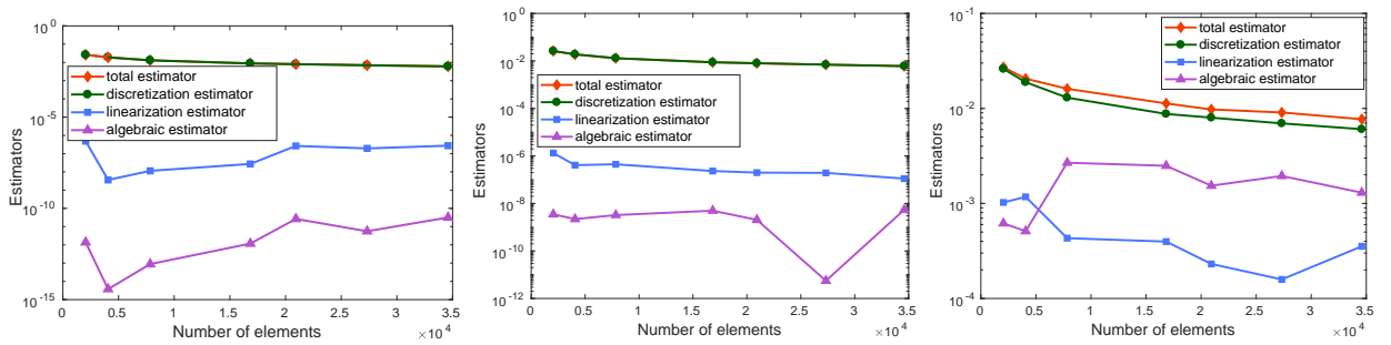
Figure 3: p = 1 : a posteriori estimators \eta_{\bar{k},\bar{i}}, \eta_{\text{disc}}, \eta_{\text{lin}}, \eta_{\text{alg}} at convergence as a function of the number of mesh elements. Exact (left), inexact (middle), and adaptive inexact (right) Newton-min methods with respectively the stopping criteria (84), (85), and (63). The log scales are different in each graph.
