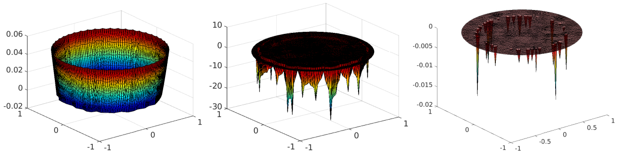
Figure 2: Left: u_{1h}^{k,i} - u_{2h}^{k,i} at the second Newton-min step ( p = 1, k = 2, i = 20 ). Center: \lambda_h^{k,i} at the third Newton-min step ( p = 2, k = \bar{k}, i = \bar{i} ); in figures, \mathbb{P}_2 functions are plotted as \mathbb{P}_1 functions on a refined mesh (each triangle divided into 4 triangles).
