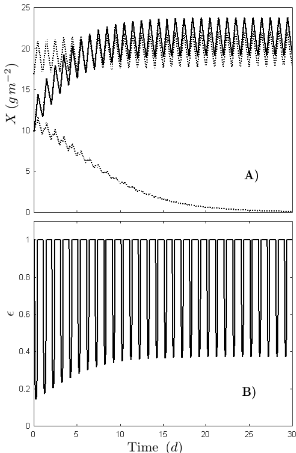
Fig. 5. A) Comparison of the evolution of biomass concentration of the controlled culture (continuous line) and the non-controlled culture (dotted line) for different initial concentrations at a dilution rate D = 0.3d^{-1} . B) Evolution of the exposure factor.
