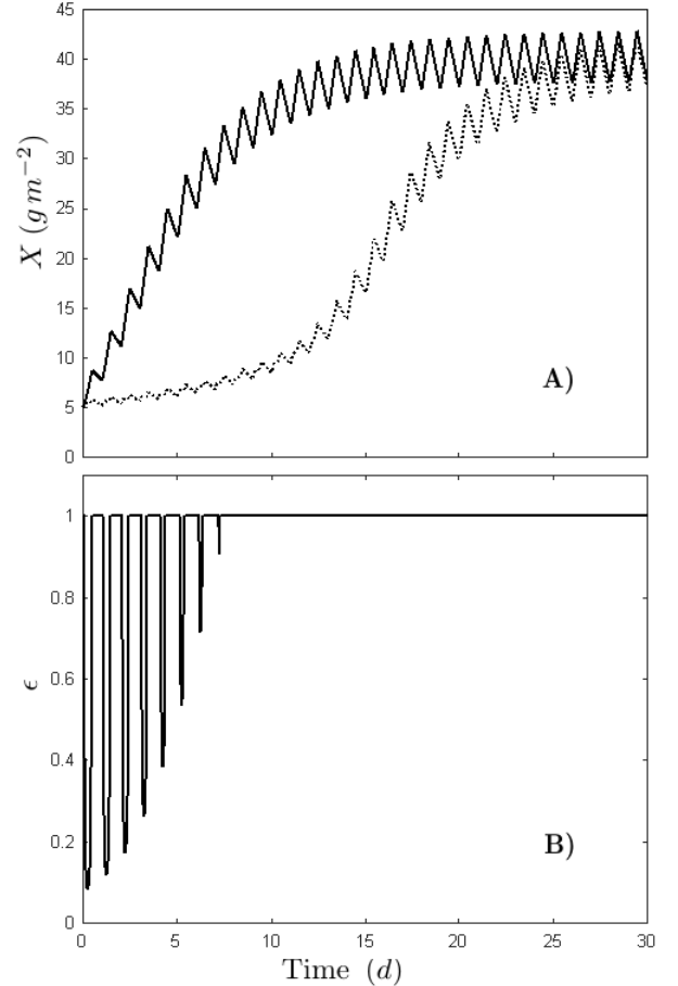
Fig. 4. A) Comparison of the evolution of biomass concentration of the controlled culture (continuous line) and the non-controlled culture (dotted line) at a dilution rate D = 0.13 \text{ d}^{-1} . B) Evolution of the exposure factor.
