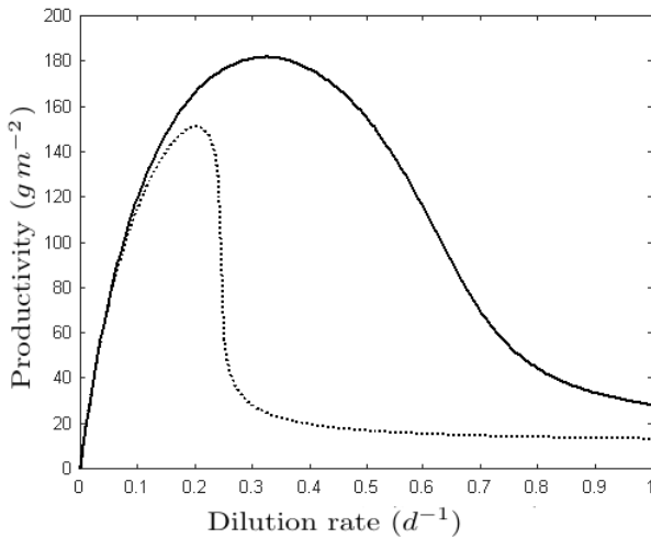
Fig. 3. Biomass productivities of the controlled culture (continuous line) and the non-controlled culture (dotted line) at different dilution rates.
