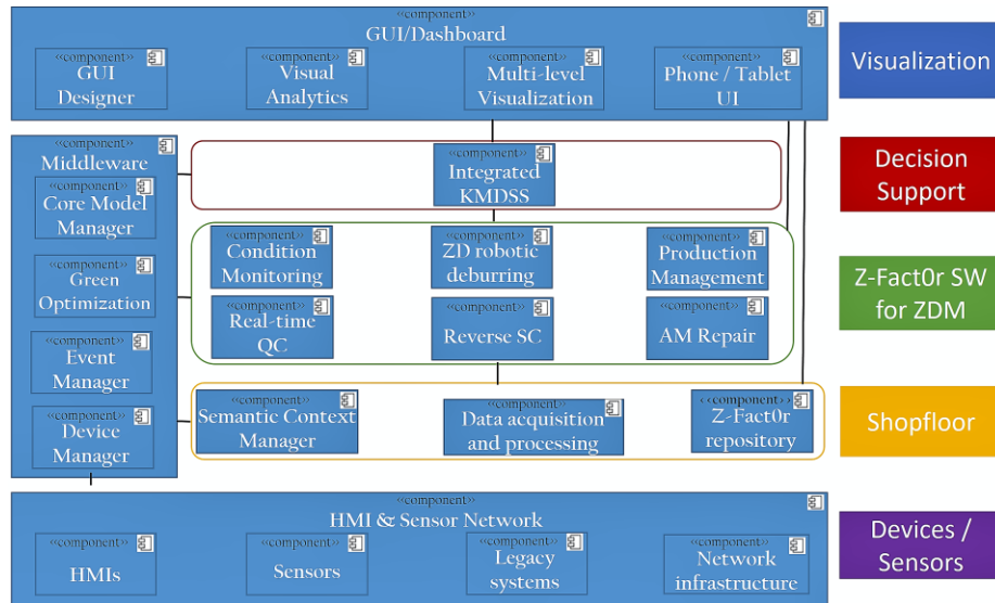
Fig. 3. Z-Fact0r functional architecture viewpoint
