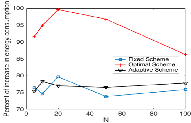
Figure 21: Comparison of the increase in energy consumption in noisy channels among transmission strategies.
