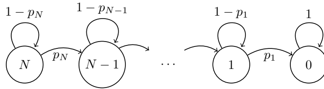
Figure 1: The Markov chain W .
