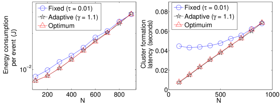
Figure 20: Comparison of simulation results for different transmission strategies.
