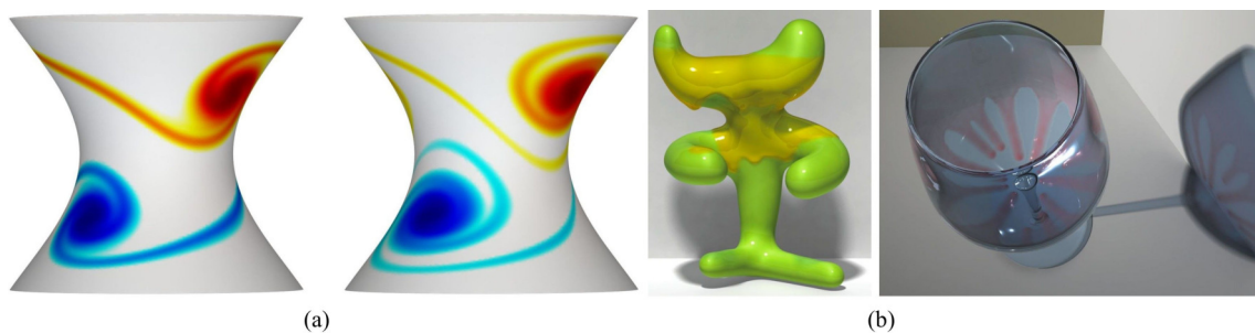
Figure 6.6: Using the functional flow for fluid simulation. (a) Simulating turbulent flow by transporting the vorticity of the fluid. (b) Simulating viscous thin film flow by transporting the mass density (visualized as an offset surface).
