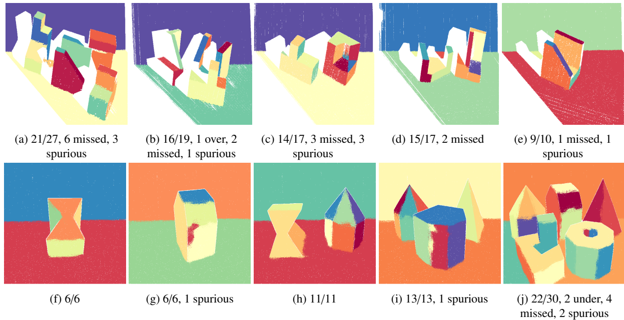
Figure 2: Results from the SegComp benchmark using RPL-GMR. Examples from ABW test data (top row) and from the PERCEPTION test data (bottom row).
