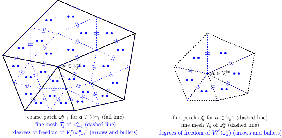
Figure 3: Degrees of freedom of the local Raviart–Thomas–Nédélec spaces \mathbf{V}_j^p(\omega_{j-1}^a) for the residual liftings \boldsymbol{\sigma}_{j,\text{alg}}^a , 1 \leq j \leq J , (left) and \mathbf{V}_h^{p'}(\omega_h^a) for the discretization flux reconstruction \boldsymbol{\sigma}_{h,\text{dis}}^a (right). Interior vertex \mathbf{a} , polynomial degree p = 1 , and discretization flux reconstruction degree p' = p = 1 .
