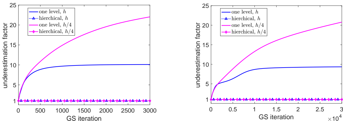
Figure 1: L-shape problem with random initial error and the Gauss–Seidel iterative solver. Underestimation of the guaranteed lower bound on the algebraic error \eta_{\text{alg}} given by (7.5a) with the one-level algebraic residual lifting of Remark 5.2 and by the hierarchical algebraic residual lifting of Definition 5.1. Mesh sizes h and h/4 , polynomial degrees p = 1 (left) and p = 3 (right). Optimal underestimation stays close to one.
