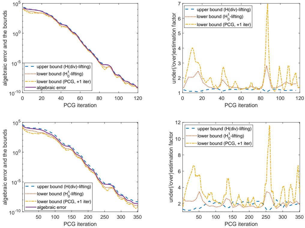
Figure 2: Porous medium flow (C.1) leading to (2.2). Conjugate gradient solver with incomplete Cholesky preconditioning. The algebraic error \|P_{\mathbf{w}}^{n,k} - P_{\mathbf{w}}^{n,k,i}\|_{\mathbb{P}_{\mathbf{w}_h}^{n,k-1}} on iteration i , the estimator (lower bound) based on comparison of two consecutive iterates \|P_{\mathbf{w}}^{n,k,i+1} - P_{\mathbf{w}}^{n,k,i}\|_{\mathbb{P}_{\mathbf{w}_h}^{n,k-1}} , the guaranteed lower bound \underline{\eta}_{\text{alg}}^i = (r_h^i, \rho_{h,\text{alg}}^i) / \|(\mathbf{A}^{n,k-1})^{\frac{1}{2}} \nabla \rho_{h,\text{alg}}^i\| on the algebraic error proposed in this paper, and the guaranteed upper bound \bar{\eta}_{\text{alg}}^i = \|(\mathbf{A}^{n,k-1})^{-\frac{1}{2}} \boldsymbol{\sigma}_{h,\text{alg}}^i\| on the algebraic error proposed in this paper (left). Corresponding effectivity indices (right). Setting of [83, Section 6.2], time step 260 (time 2.6 \cdot 10^6 s), first iterative coupling linearization, 45 \times 45 mesh (top) and 137 \times 137 mesh (bottom).
