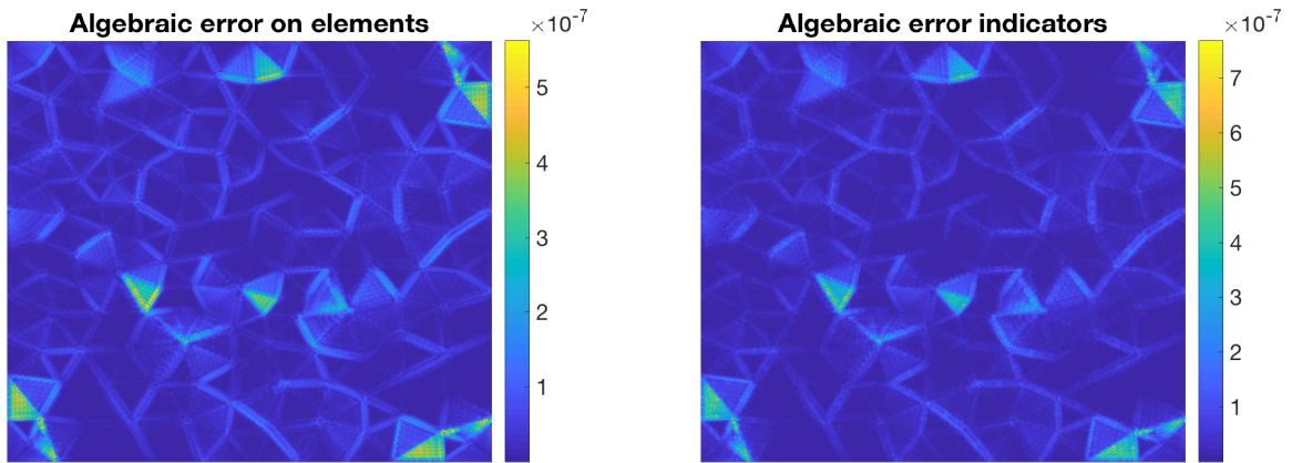
Figure 6: Sinus problem, p = 2 : elementwise distribution of the algebraic energy error \|\nabla(u_h^{\text{ex}} - u_h)\|_K (left) and of the local error indicators \bar{\eta}_{\text{alg},K} (right) after one full multigrid cycle
