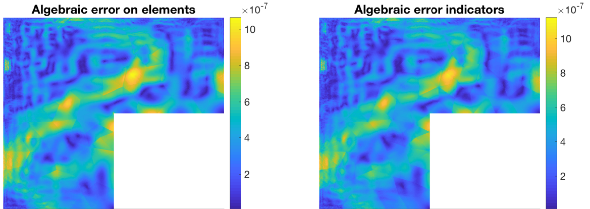
Figure 10: L-shape problem, p = 3 : elementwise distribution of the algebraic energy error \|\nabla(u_h^{\text{ex}} - u_h)\|_K (left) and of the local error indicators \bar{\eta}_{\text{alg},K} (right) after 28 PCG iterations
