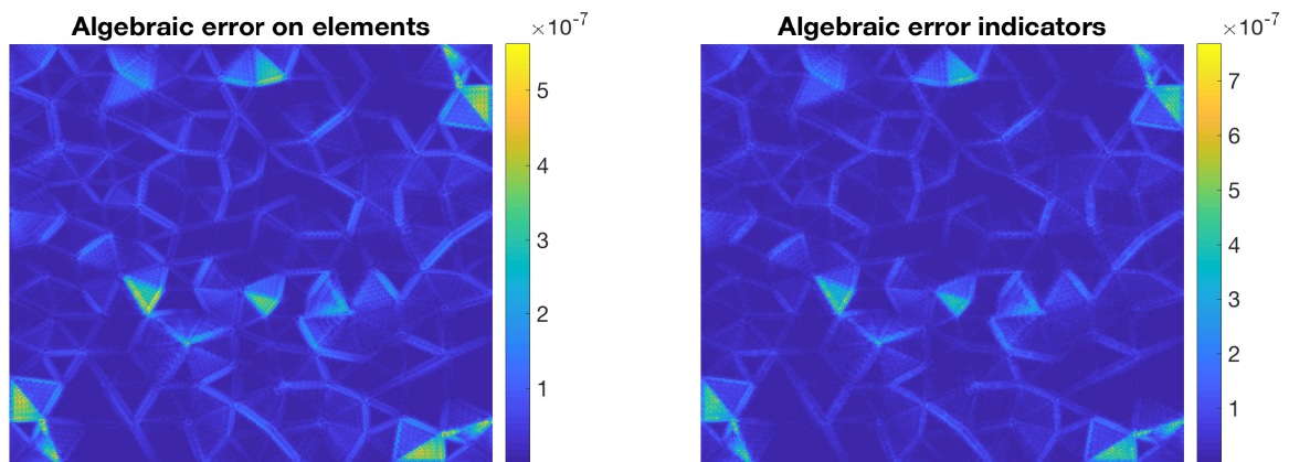
Figure 6: Sinus problem, p = 2 : elementwise distribution of the algebraic energy error \|\nabla(u_h^{\text{ex}} - u_h)\|_K (left) and of the local error indicators \bar{\eta}_{\text{alg},K} (right) after one full multigrid cycle
