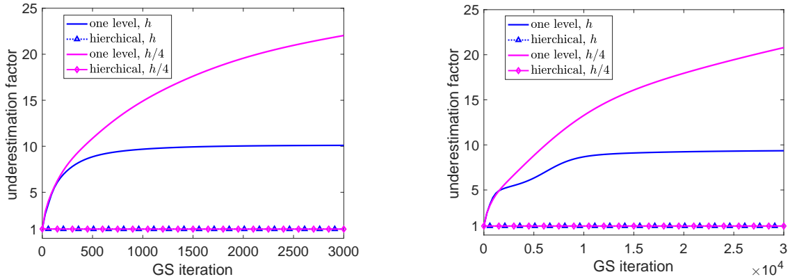
Figure 1: L-shape problem with random initial error and the Gauss–Seidel iterative solver. Underestimation of the guaranteed lower bound on the algebraic error \underline{\eta}_{\text{alg}} given by (7.5a) with the one-level algebraic residual lifting of Remark 5.2 and by the hierarchical algebraic residual lifting of Definition 5.1. Mesh sizes h and h/4 , polynomial degrees p = 1 (left) and p = 3 (right). Optimal underestimation stays close to one.
