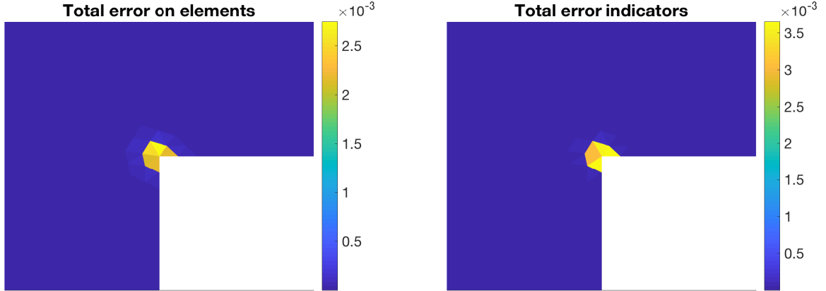
Figure 9: L-shape problem, p = 3 : elementwise distribution of the total energy error \|\nabla(u - u_h)\|_K (left) and of the local error indicators \eta_K (right) after 28 PCG iterations. We plot in both figures the part [-0.1, 0.1] \times [-0.1, 0.1] of the discretization domain \Omega
