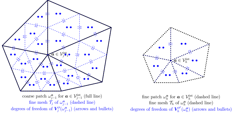
Figure 3: Degrees of freedom of the local Raviart–Thomas–Nédélec spaces \mathbf{V}_j^p(\omega_{j-1}^a) for the residual liftings \sigma_{j,\text{alg}}^a , 1 \leq j \leq J , (left) and \mathbf{V}_h^{p'}(\omega_h^a) for the discretization flux reconstruction \sigma_{h,\text{dis}}^a (right). Interior vertex \mathbf{a} , polynomial degree p = 1 , and discretization flux reconstruction degree p' = p = 1 .
