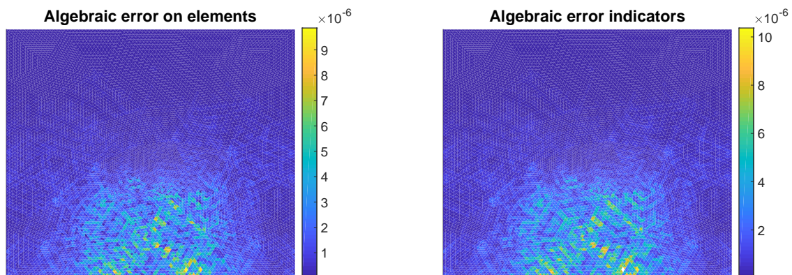
Figure 8: Peak problem, p = 1 : elementwise distribution of the algebraic energy error \|\nabla(u_h^{\text{ex}} - u_h)\|_K (left) and of the local error indicators \bar{\eta}_{\text{alg},K} (right) after 2 iterations of the multigrid V-cycle
