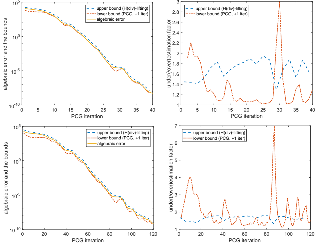
Figure 2: Porous medium flow (C.1) leading to (2.2). Conjugate gradient solver with incomplete Cholesky preconditioning. The algebraic error \|P_w^{n,k} - P_w^{n,k,i}\|_{\mathbb{P}_w^{n,k-1}} on iteration i , the estimator (lower bound) based on comparison of two consecutive iterates \|P_w^{n,k,i+1} - P_w^{n,k,i}\|_{\mathbb{P}_w^{n,k-1}} , and the guaranteed upper bound \bar{\eta}_{\text{alg}}^i = \|(\mathbf{A}^{n,k-1})^{-\frac{1}{2}} \boldsymbol{\sigma}_{h,\text{alg}}^i\| on the algebraic error proposed in this paper (left). Corresponding effectivity indices (right). Setting of [72, Section 6.2], time step 260 (time 2.6 \cdot 10^6 s), fist iterative coupling linearization, 15 \times 15 mesh (top) and 45 \times 45 mesh (bottom).
