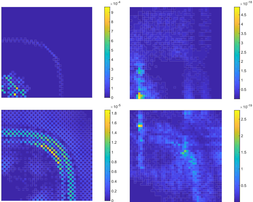
Figure 11: Recovering mass balance on each step (C.5) of a combined temporal/spatial/linearization/algebraic algorithm for numerical approximation of (C.1). Data and setting of [72, Section 6.1], 45 \times 45 uniform mesh, time step 260 (time 2.6 \cdot 10^6 s), fist Newton linearization, iteration 195 of GMRes solver with diagonal preconditioning, adaptive stopping criterion [72, (4.13a)] with \gamma_{\text{alg}} = 0.001 . Original mass balance misfit in each computational cell in \text{m}^2\text{s}^{-1} (left), corrected mass balance misfit in \text{m}^2\text{s}^{-1} (right). Water phase (top), oil phase (bottom). Please note the difference in the scales.
