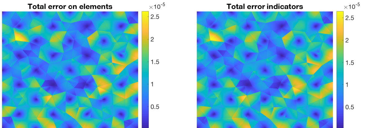
Figure 5: Sinus problem, p = 2 : elementwise distribution of the total energy error \|\nabla(u - u_h)\|_K (left) and the of local error indicators \eta_K (right) after one full multigrid cycle
