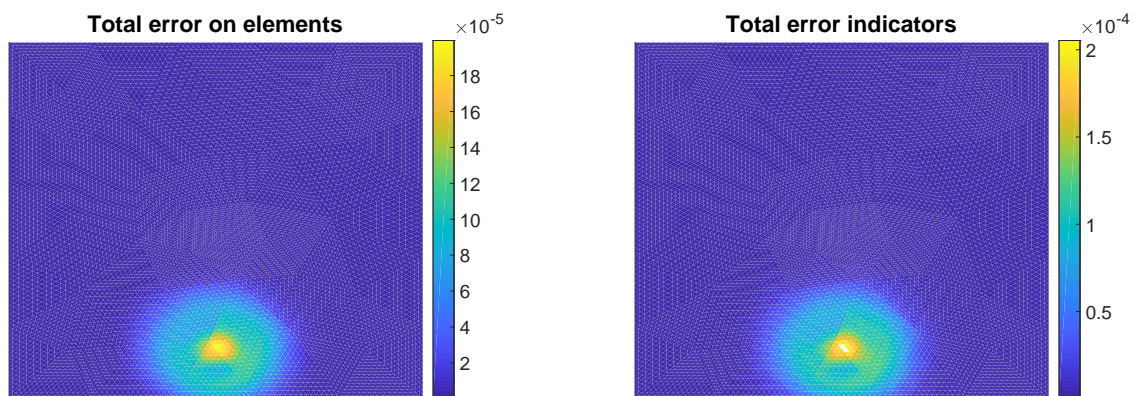
Figure 7: Peak problem, p = 1 : elementwise distribution of the total energy error \|\nabla(u - u_h)\|_K (left) and of the local error indicators \eta_K (right) after 2 iterations of the multigrid V-cycle
