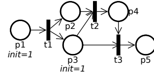
Figure 2: Concrete syntax representation of a Petri net model conforming to the abstract syntax of the DSL from Figure 1.
