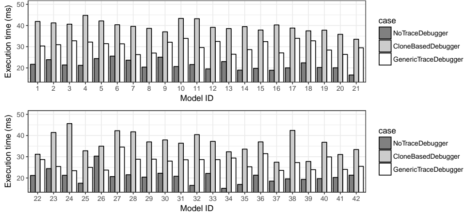
Figure 16: Time required to explore all future states with the set of 42 small models from industrial sources (34 to 61 objects per model).
