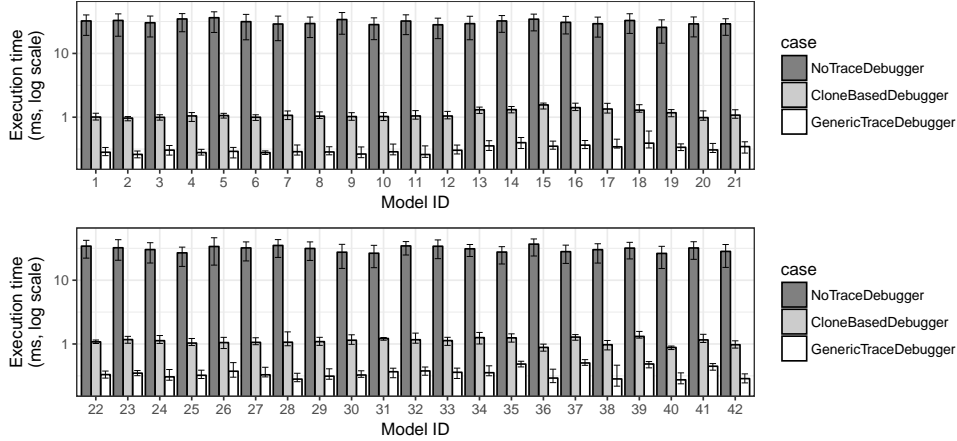
Figure 14: Time required to explore one past state with the set of 42 small models from industrial sources (34 to 61 objects per model).
