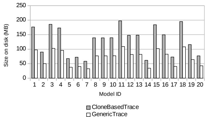
Figure 13: Size on disk of execution traces, with the set of 20 randomly generated large models (500 to 1000 objects per model)
