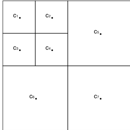
Figure 5: Discretization grid of the Laplacian in c_4
