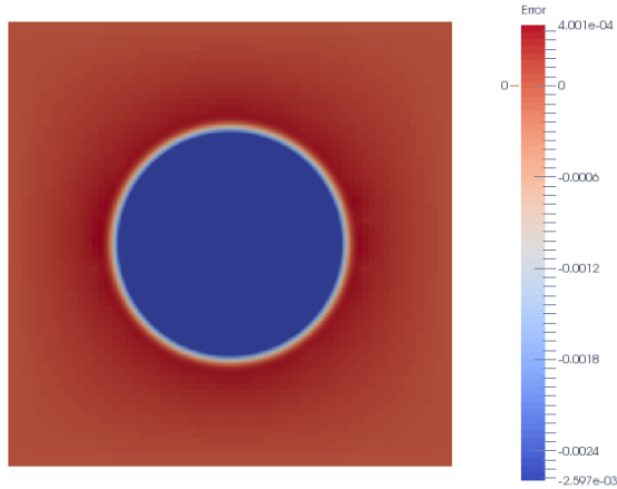
Figure 19: Mesh referring to table 11. Error distribution.
