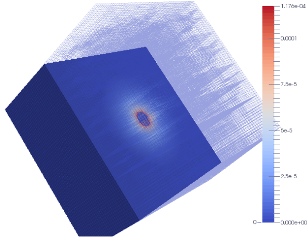
Figure 27: Error distribution in a cross section for the 3D penalized sphere test case.
