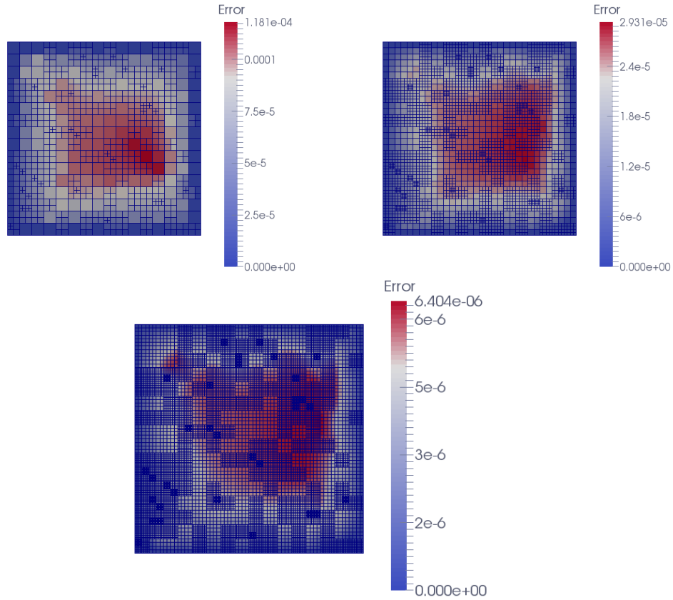
Figure 9: Error distribution for random mesh generation. Levels 6,7 and 8 respectively.
