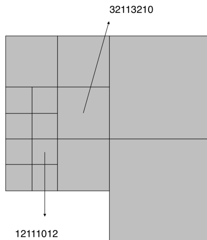
Figure 4: Example of bijective key construction.
