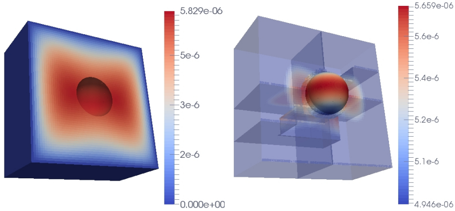
Figure 23: Distribution of the errors for a mesh refinement with level 9 inside the sphere and 6 outside for 2D u_e(x, y, z) = \sin((x - 0.5)^2 + (y - 0.5)^2) .
