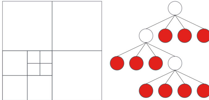
Figure 2: A square decomposition and the corresponding quadtree.
