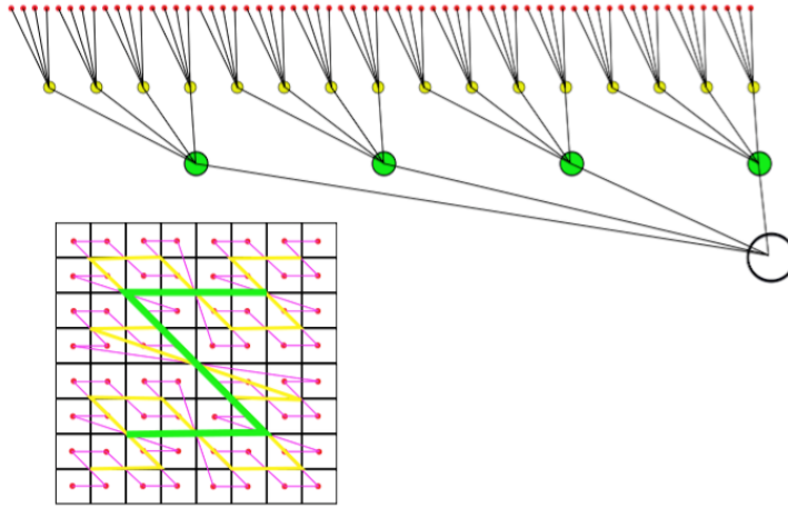
Figure 3: Global nested Z-ordering example.
