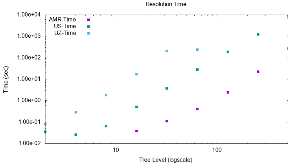
Figure 13: Resolution time trend.
