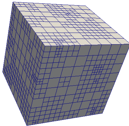
Figure 25: Random mesh generation: initial grid.
