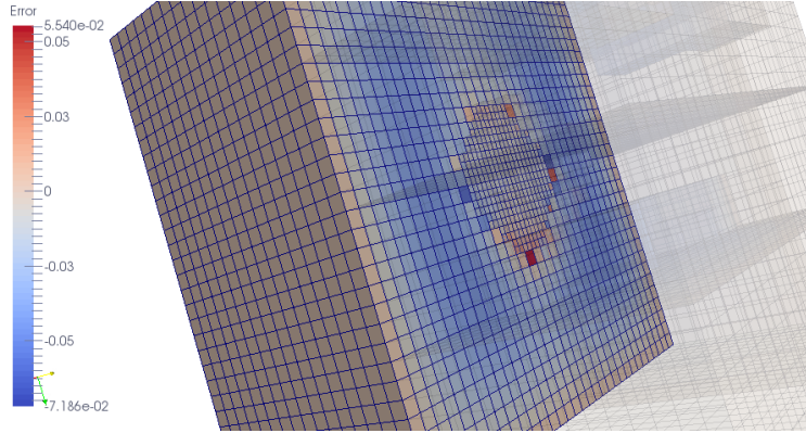
Figure 21: Error map on a cross section for u_e(x, y, z) = \sin((x - 0.5)^2 + (y - 0.5)^2) with 2:1 refinement in a sphere.
