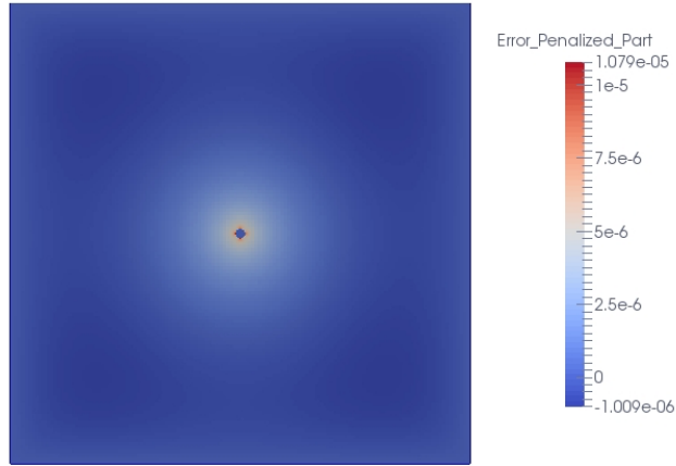
Figure 11: Error distribution on the whole domain for the penalized cylinder with radius equal to 0.01.
