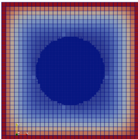
Figure 17: Error example, level 8, sinus analytical function.
