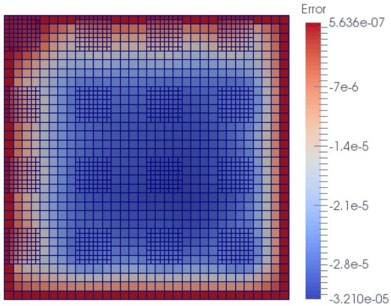
Figure 8: Example of error distribution on a grid corresponding to level 6.
