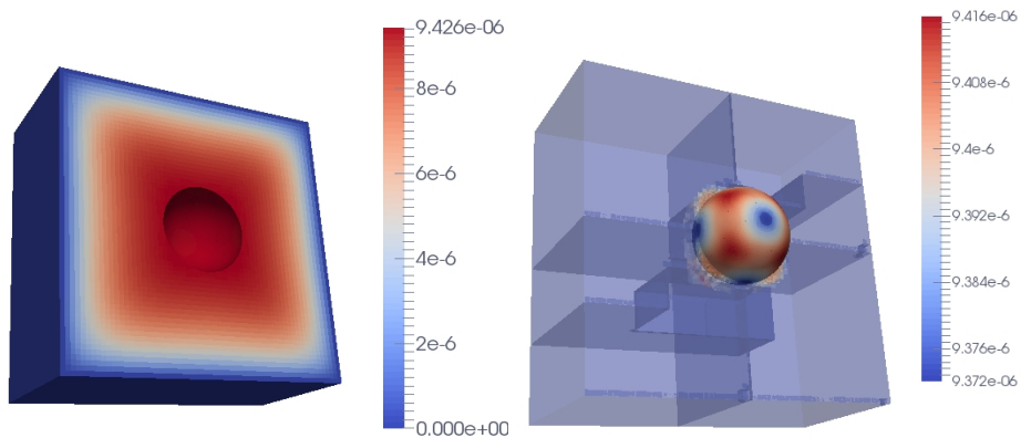
Figure 24: Distribution of the errors for a mesh refinement with level 9 inside the sphere and 6 outside for 3D sinus analytical function.
