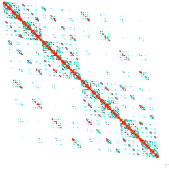
Figure 20: Structure of the 3D matrix for the Laplacian operator with 2:1 graded grid (36128 points).
