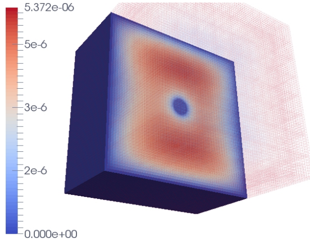
Figure 26: Error distribution in a cross section for the 3D penalized sphere test case.
