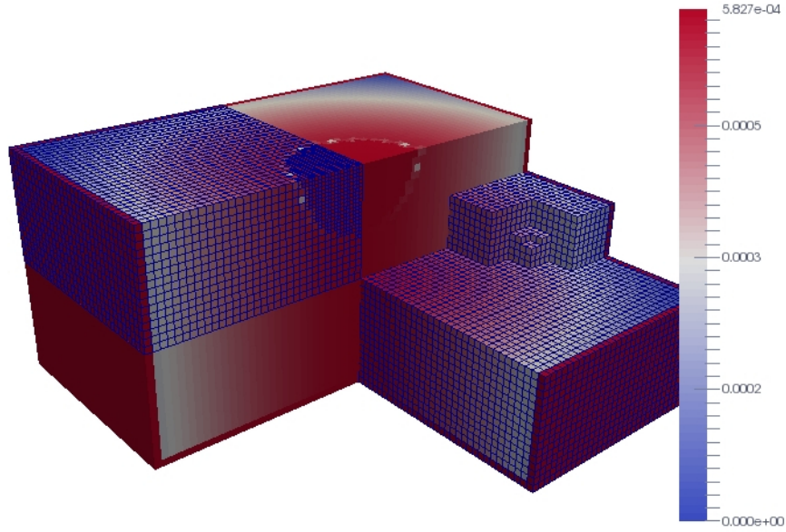
Figure 22: Representation of the residuals for the 3D Laplace operator in several cross sections.
