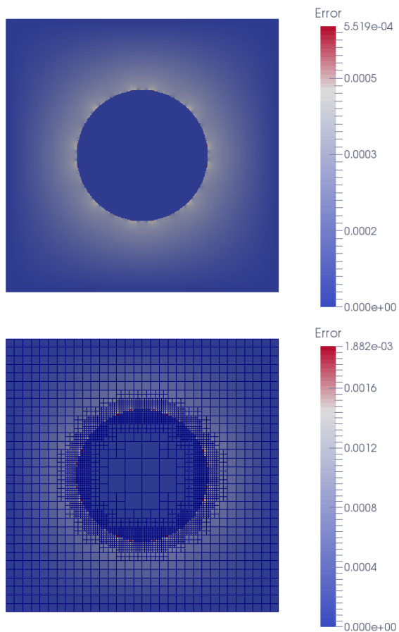
Figure 10: Error distribution for the penalized cylinder with a maximum tree level 9 and 7 respectively.
