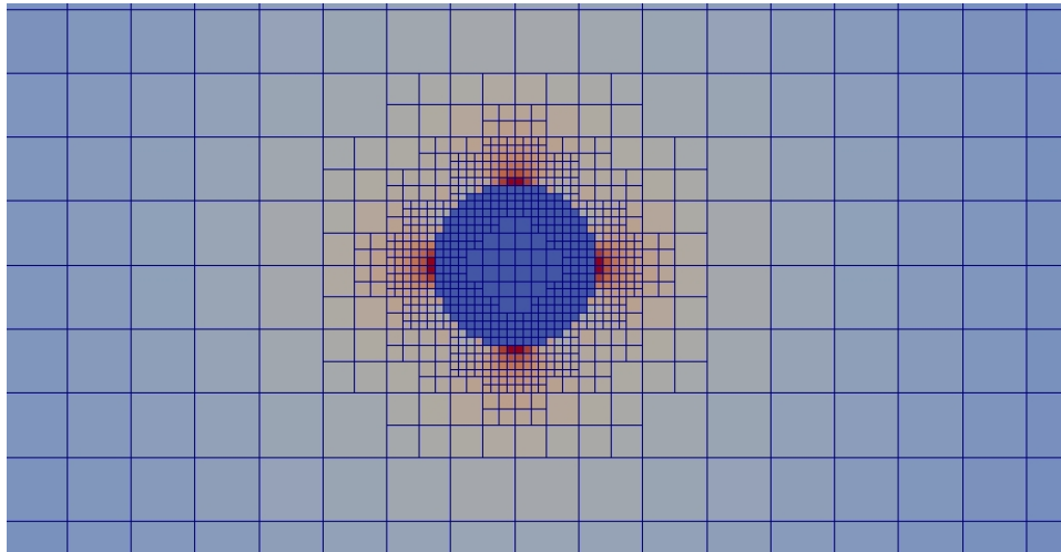
Figure 11: Error distribution on the whole domain for the penalized cylinder with radius equal to 0.01.
