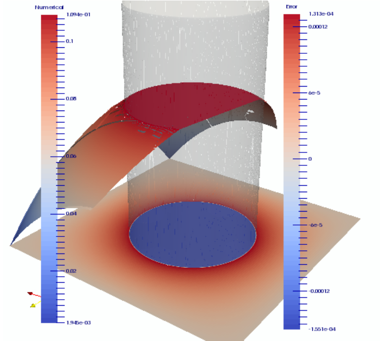
Figure 14: Numerical result obtained by AMR, superposition of analytical and numerical solution plane section, with a projection of the error and a representation of the mollification (grey part).
