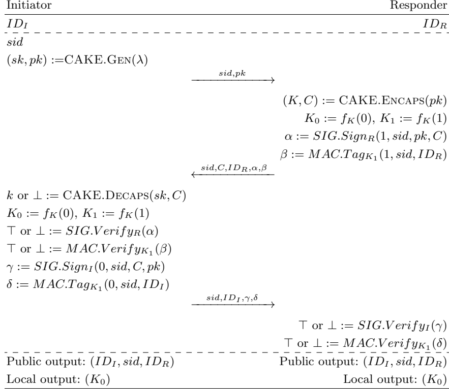
Fig. 2: SIGMA-like Authenticated Key Exchange From CAKE KEM
