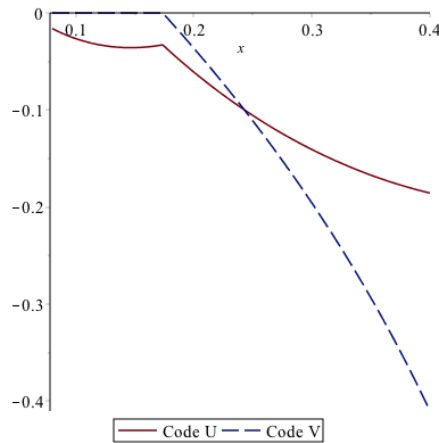
Fig. 5. \alpha_{(U,U)}(w/n) and \alpha_{(\mathbf{0},V)}(w/n) against x \triangleq \frac{w}{n} .
