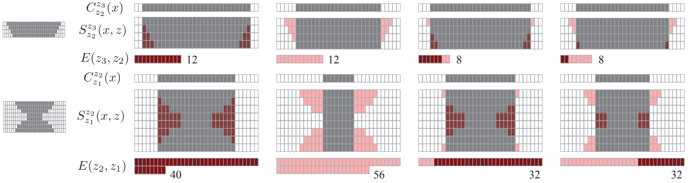
Fig. 3. The geometry of a slice is obtained by extruding its image along the z -axis, i.e. slices are approximated to have vertical walls. This results in an approximation error, as some grid cells that belong to the inside of the object are not part of a slice (light red) and some grid cells that belong to the exterior are part of a slice (dark red). The error of a slice is the number of wrongly classified grid cells. Using the midlevel contour for approximation is optimal only if a ray along the z direction intersects the geometry not more than once (compare upper vs. lower row). The optimal contour is not necessarily unique (slices on the right).
