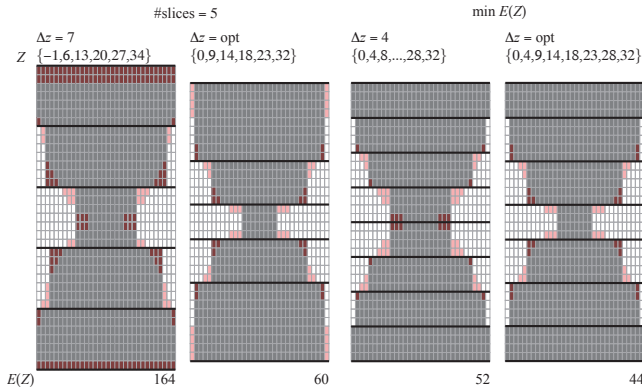
Fig. 6. Slicing the hourglass shape – uniform vs. optimal. The left results are generated with a target of 5 slices. Uniform slicing leads to overestimating the shape, resulting in large volumetric error. Optimal slicing provides a significantly better result using the same number of slices and a minimal slice thickness of 4. On the right we show the best uniform result for a minimum slice thickness of 4 as well as an optimal slicing having smaller error while using one slice less.
