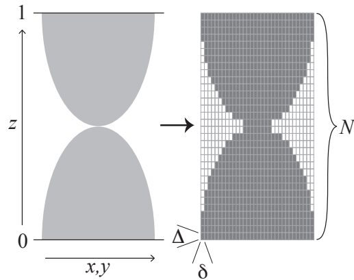
Fig. 1. The input shape \mathcal{S} is assumed to cover [0, 1] in direction \mathbf{z} . The shape is discretized and represented on an occupancy grid with grid constant \Delta = 1/N in direction \mathbf{z} , where N is the number of layers along z covering the shape; and grid constant \delta in the directions \mathbf{x} and \mathbf{y} .
