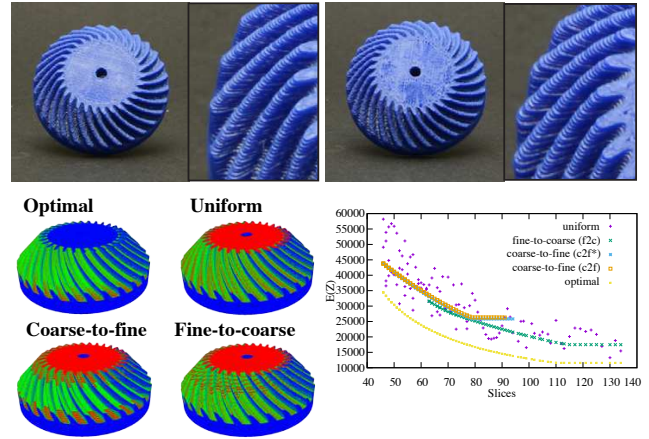
Fig. 10. Top: (Left) Optimally sliced gear model with layer heights between 0.1 - 0.3\text{mm} and E(Z) = 22007.85 . (Right) Uniformly sliced with a layer height of 0.214 and E(Z) = 39122.30 . Both prints have 64 slices. Bottom: The error maps illustrate that optimal slicing does not generate errors in the top region of the model where other adaptive schemes fail to faithfully reproduce the correct height of the model.
