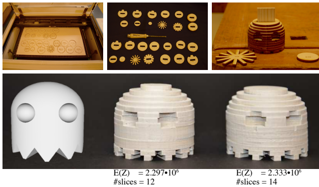
Fig. 11. Shape manufactured by cutting pieces from plywood that are stacked, glued, and spray painted to generate the physical artifact. The final result on the left shows optimal slicing, using 4,8 and 10mm sheets. Finest uniform slicing (final result on the right) only uses the 4mm plywood. Optimal slicing has slightly smaller volumetric error and better reproduces the desired height of the shape. We also prefer the visual appearance of optimal slicing, as it better reproduces the eyes and the round top.
