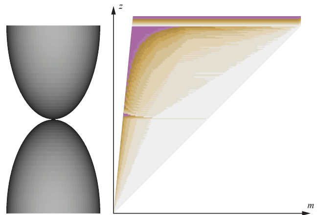
Fig. 5. The table of thicknesses generated by dynamic programming for an hourglass shape. Thickness is color-coded, starting with light gray for the thinnest available slice. The smaller slopes towards the center of the shape require thinner slices. This shows in the table as larger portions of each row being assigned to thinner slices, in particular the larger amount of light gray. The center itself, however, is better covered with one thicker slice.
