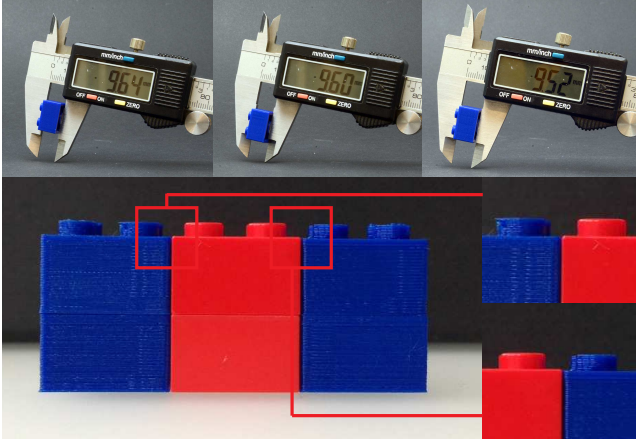
Fig. 9. Top: Uniformly sliced Lego brick with layer height of 0.099375\text{mm} (Left). Adaptively sliced brick using layer height between 0.05 - 0.2\text{mm} (Middle). Uniformly sliced brick with layer height of 0.19875\text{mm} . Bottom: Optimal sliced and 3D printed Lego bricks (left) reproduces the height of real bricks (middle) more closely than uniformly sliced ones (right) printed in the same time.
