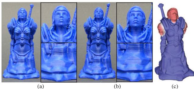
Fig. 12. Importance map specifies where the slicer has to use thinner slices to lower the error in these areas. This example consists of 550 slices with slice heights between 0.1mm to 0.3mm. (Left: Adaptive slicing without importance values, Middle: Adaptive slicing including importance map. Right: User-defined importance map.
