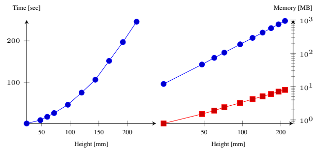
Fig. 8. Computational resources relative to the resolution for the 3DBENCHY. The left plot shows computation times and the right plots uncompressed and compressed data, both relative to the height of the shape for fixed FDM parameters. Adjusting the height for fixed \Delta is roughly equivalent to varying \Delta for fixed height. Note that storage requirements also change from quadratic in the uncompressed case to linear for the compressed version.
