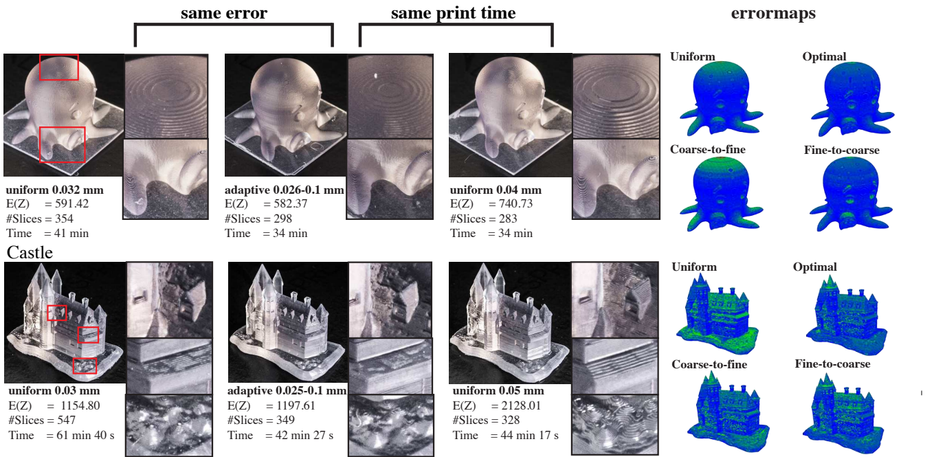
Fig. 14. 3D printed stereolithography results. High-resolution uniform slicing (column 1), Optimal discrete slicing with the same error (column 2), Low-resolution uniform slicing with the same printing time (column 3), error maps show the error for column 2 and 3 results and additionally for a coarse-to-fine and fine-to-coarse slicing approaches.
