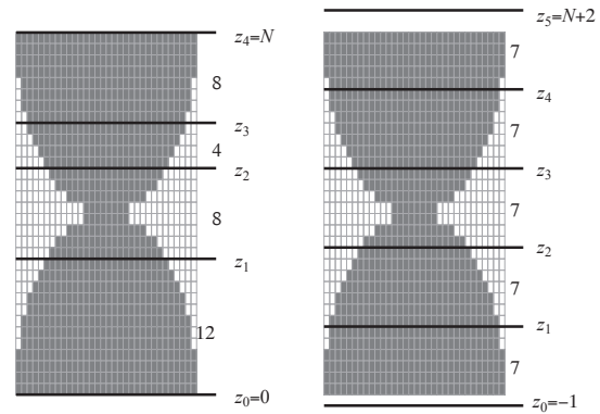
Fig. 2. A slicing is represented by the sequence Z = \{z_0, z_1, \dots, z_n\} along the \mathbf{z} -direction. The height of slices may vary (left). Admissible slice heights \mathcal{T} = \{h_0, h_1, \dots\} \in \Delta\mathbb{Z}^+ are a subset of integer multiples of \Delta so that all slice boundaries necessarily align with the grid. The slices cover the object. The first and last slice may extend beyond the shape to accommodate restrictions in the available slice heights, such as in the uniform slicing on the right.
