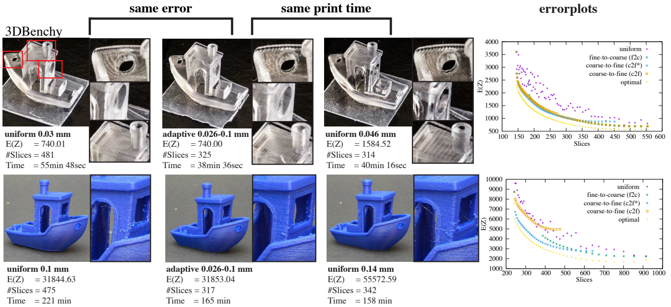
Fig. 13. We compare the same model using different 3D printing technologies. High-resolution uniform slicing (column 1), Optimal discrete slicing with the same error (column 2), Low-resolution uniform slicing with the same printing time (column 3), error plot shows different methods and their slicing errors over the number of slices. Note here, that if the number of possible slice heights is limited adaptive strategies such as c2f fail to generate longer and more accurate slice sequences.
