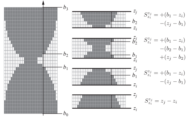
Fig. 4. Per-slice errors can be quickly updated for each location by conceptually intersecting a ray along slicing direction against the boundaries of the shape. Intersections b_0, b_1, \dots represent changes from outside to inside for even indices and from inside to outside for odd indices. The ray contributes to the error of a slice only if the slice contains any intersection. The computational complexity of computing the error is proportional to the number of intersections, and independent of the number of elements a slice contains.
