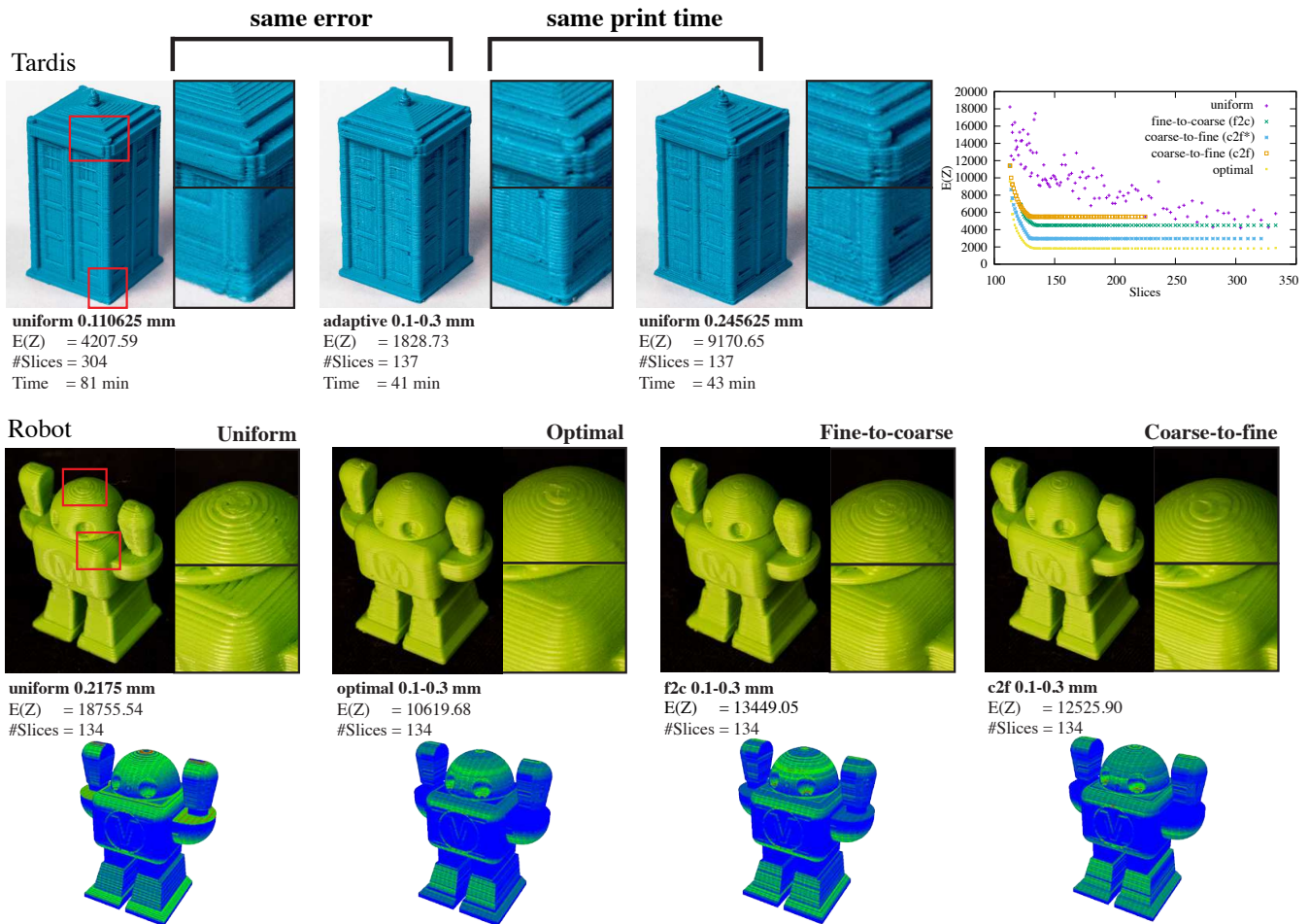
Fig. 15. 3D printed FDM results. Top row: High-resolution uniform slicing (column 1), Optimal discrete slicing with the same error (column 2), Low-resolution uniform slicing with the same printing time (column 3), error plot shows different methods and their slicing errors over the number of slices. Bottom row: Low-resolution uniform slicing (column 1), Optimal discrete slicing printed in the same time (column 2), Fine-to-coarse approach with larger overall error (column 3), Coarse-to-fine slicing (column 4) and their corresponding error maps below.
