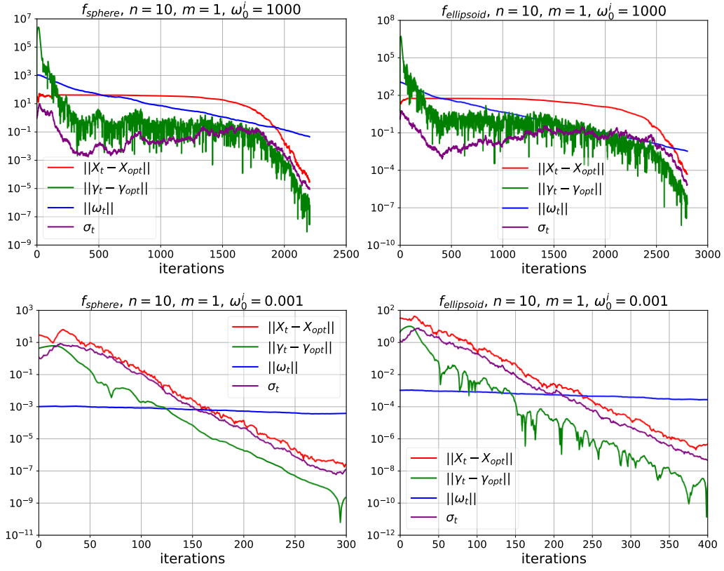
Figure C.10: Single runs on f_{\text{sphere}} (left) and f_{\text{ellipsoid}} (right) with m = 1 in n = 10 , with different values of \omega_0 .
