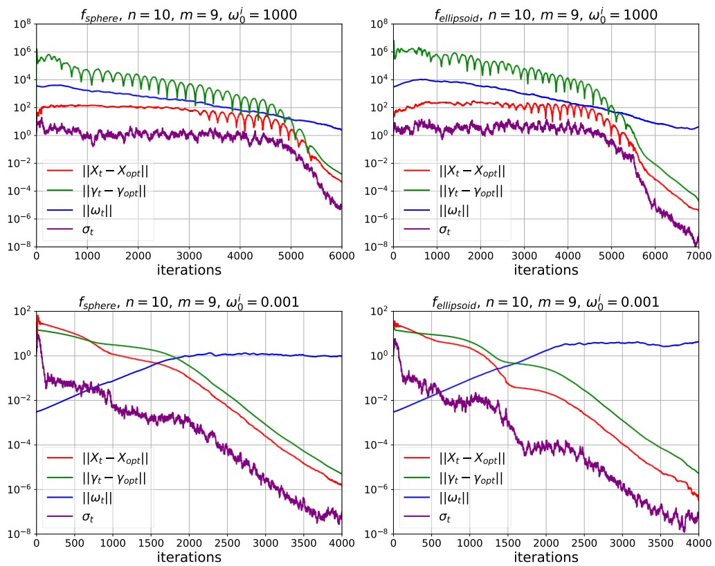
Figure C.13: Single runs on f_{\text{sphere}} (left) and f_{\text{ellipsoid}} (right) with m = 9 in n = 10 , with different values of \omega_0 .
