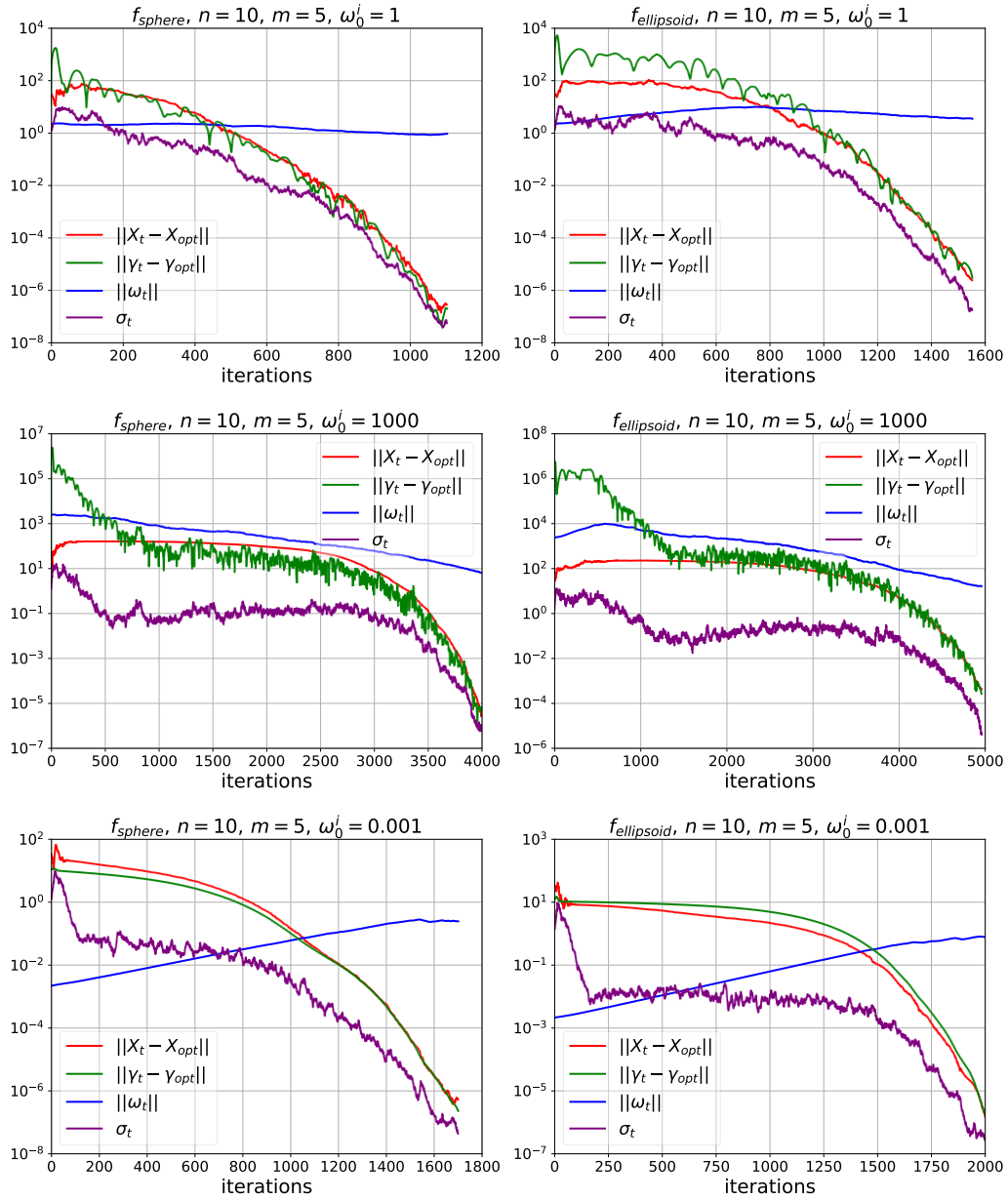
Figure C.12: Single runs on f_{\text{sphere}} (left) and f_{\text{ellipsoid}} (right) with m = 5 in n = 10 , with different values of \omega_0 .
