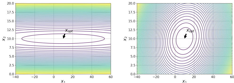
Figure 5: Contour lines of the augmented Lagrangian h corresponding to constrained f_{\text{ellipsoid}} with condition number \alpha = 10^3 in n = 2 . Left: The number of constraints m = 1 , \gamma = \gamma_{\text{opt}} = 1 , and \omega = 0 . Right: m = 2 and \gamma = \gamma_{\text{opt}} = (1, 0)^\top . \omega is set approximately to the stationary value the (\mu/\mu_w, \lambda) -CSA off -AL converges to, that is \omega = (0.05, 10^6)^\top .
