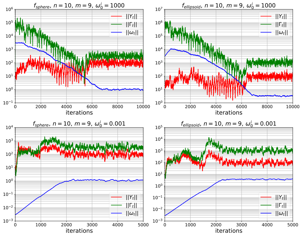
Figure C.9: Simulations of the Markov chain on f_{\text{sphere}} (left) and f_{\text{ellipsoid}} (right) with m = 9 in n = 10 .
