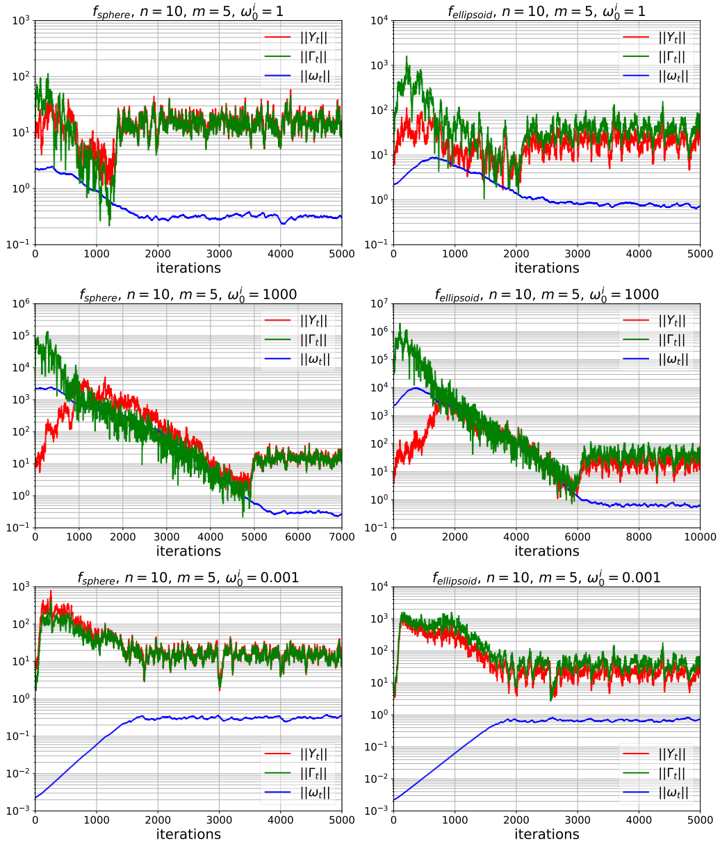
Figure C.8: Simulations of the Markov chain on f_{\text{sphere}} (left) and f_{\text{ellipsoid}} (right) with m = 5 in n = 10 .
