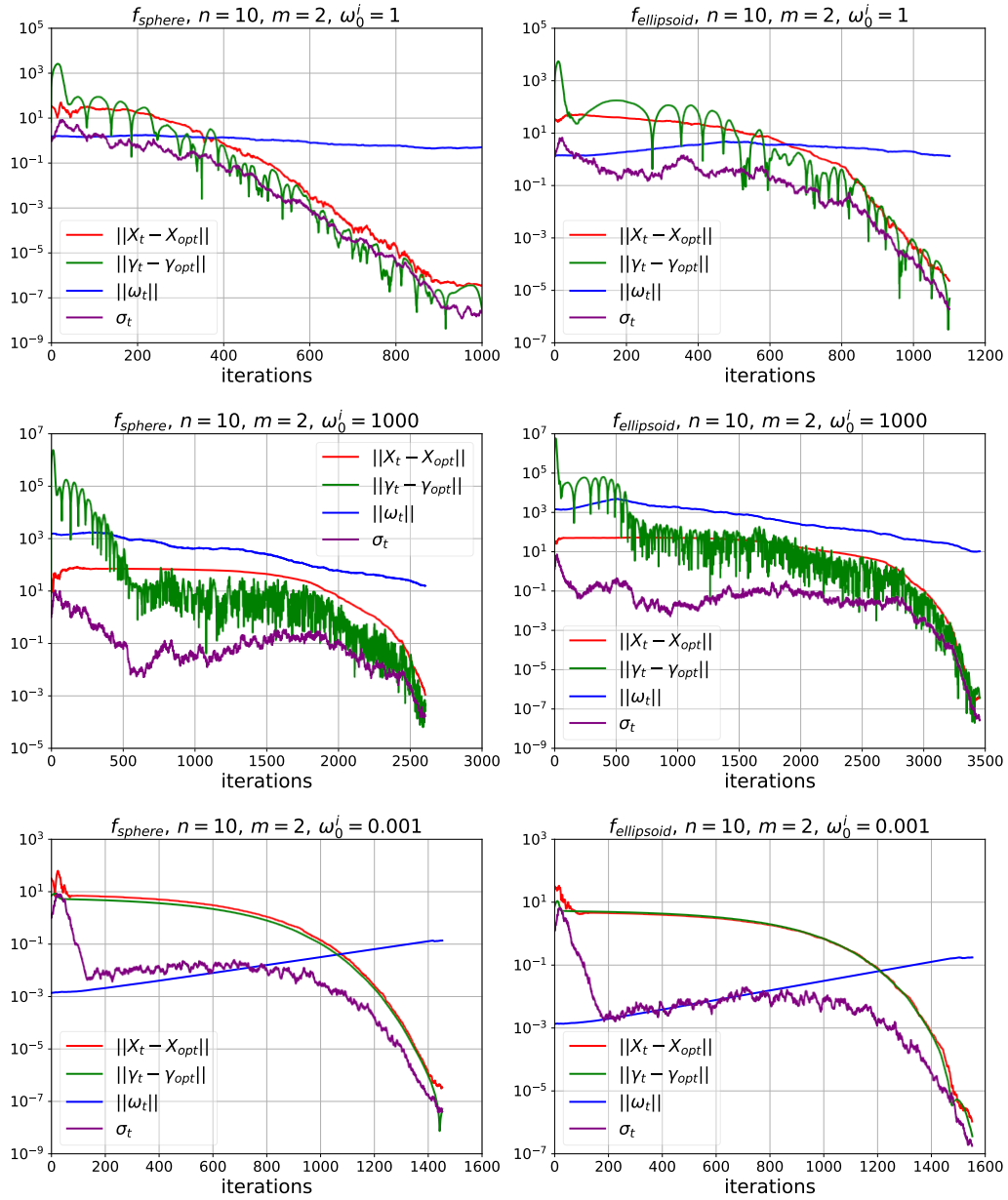
Figure C.11: Single runs on f_{\text{sphere}} (left) and f_{\text{ellipsoid}} (right) with m = 2 in n = 10 , with different values of \omega_0 .
