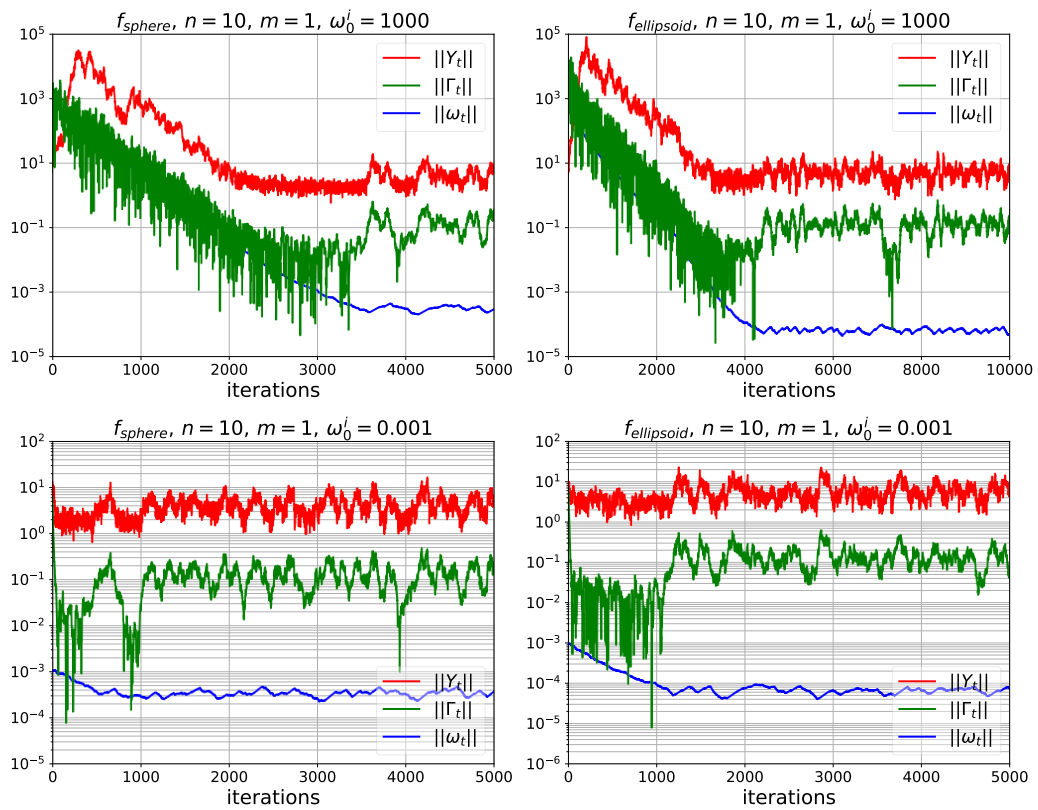
Figure C.6: Simulations of the Markov chain on f_{\text{sphere}} (left) and f_{\text{ellipsoid}} (right) with m = 1 in n = 10 .
