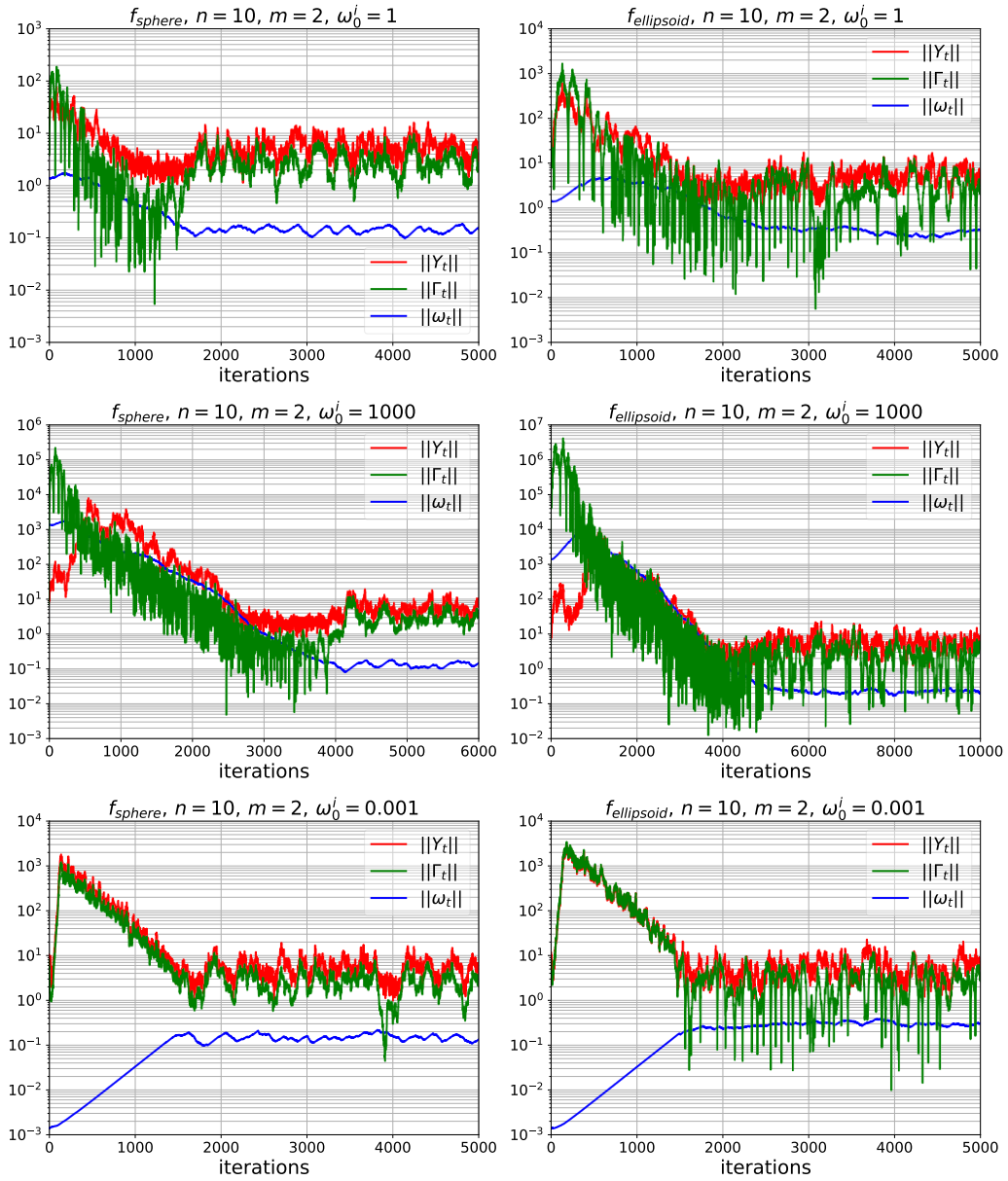
Figure C.7: Simulations of the Markov chain on f_{\text{sphere}} (left) and f_{\text{ellipsoid}} (right) with m = 2 in n = 10 .
