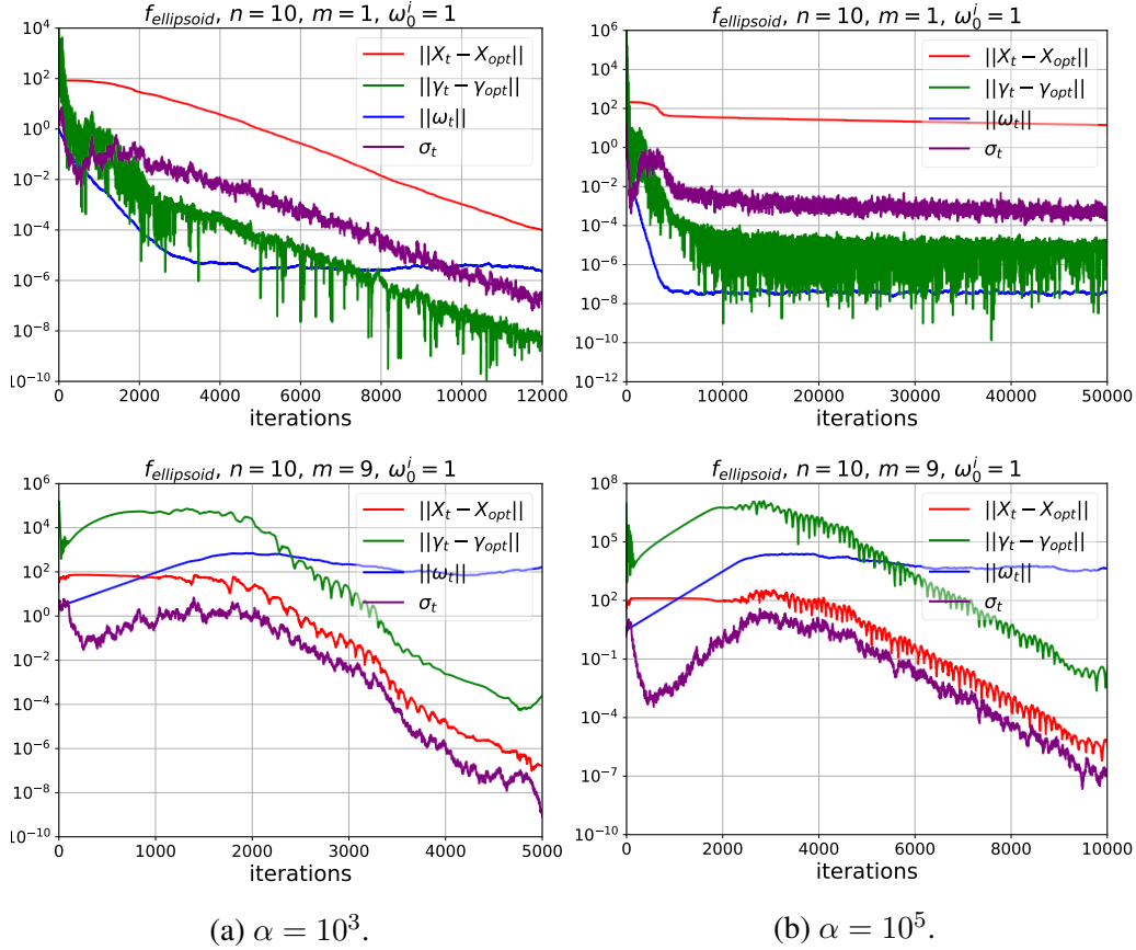
Figure 4: Single runs of the (\mu/\mu_w, \lambda) -CSA off -AL on f_{\text{ellipsoid}} with condition number \alpha = 10^3 (left) and on f_{\text{ellipsoid}} with condition number \alpha = 10^5 (right) with m = 1 (top) and m = 9 (bottom) in n = 10 .
