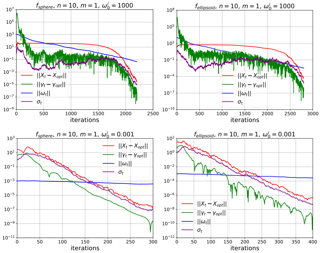
Figure C.10: Single runs on f_{sphere} (left) and f_{ellipsoid} (right) with m = 1 in n = 10 , with different values of \omega_0 .
