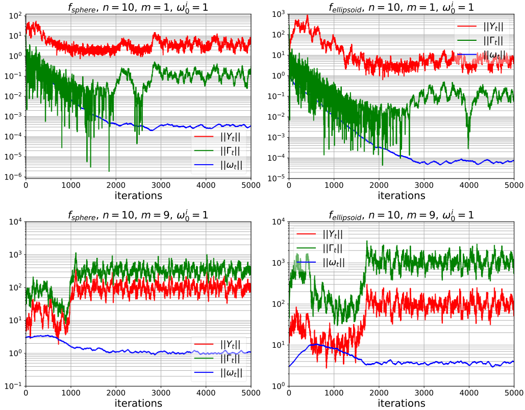
Figure 2: Simulations of the Markov chain on f_{\text{sphere}} (left) and f_{\text{ellipsoid}} (right) with m = 1 (top) and m = 9 (bottom) in n = 10 .
