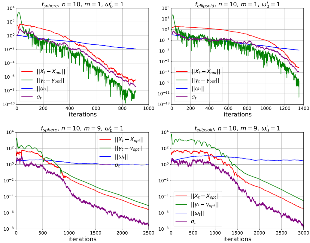
Figure 3: Single runs of the (\mu/\mu_w, \lambda) -CSA off -AL on f_{\text{sphere}} (left) and f_{\text{ellipsoid}} (right) with m = 1 (top) and m = 9 (bottom) in n = 10 .
