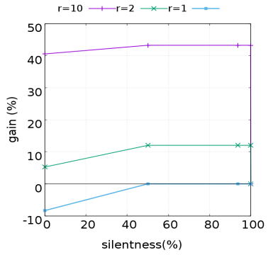
(a) backprop
