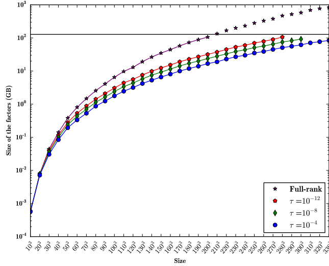
Figure 10: Memory scalability with three tolerance thresholds for the Minimal Memory /RRQR scenario when increasing the size of 3D Laplacians.
