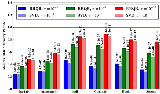
Figure 9: Memory peak for the Minimal Memory scenario with three tolerance thresholds and both SVD and RRQR kernels.
