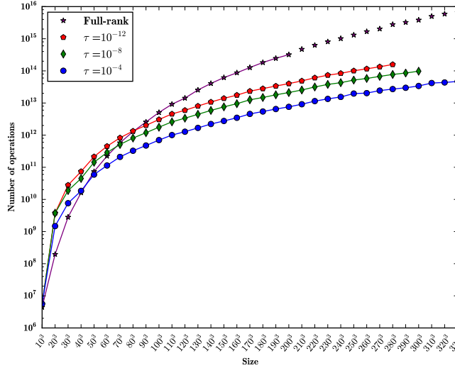
Figure 11: Number of operations scalability with three tolerance thresholds for the Minimal Memory /RRQR scenario when increasing the size of 3D Laplacians.
