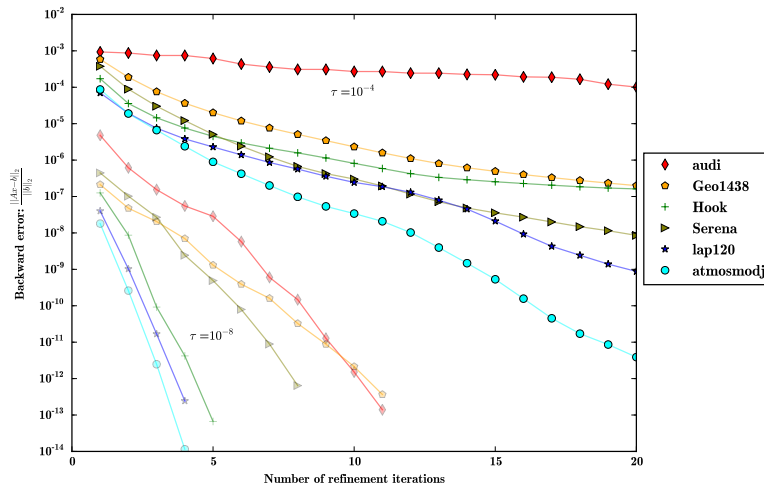
Figure 12: Convergence speed for the Minimal Memory /RRQR scenario with two tolerance thresholds.
