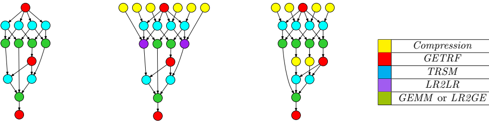
Figure 4: Full-rank. Figure 5: Minimal Memory . Figure 6: Just-In-Time .
