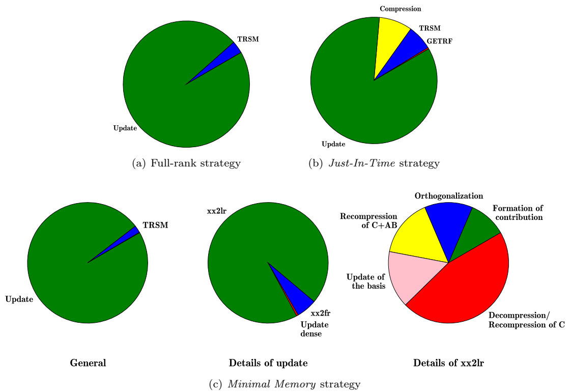
Figure 14: Breakdown of the most time-consuming kernels for the full-rank strategy ( top-left ), the Just-In-Time strategy ( top-right ), and the Minimal Memory strategy ( bottom ) on the atmosmodj case using the RRQR kernels with \tau = 10^{-8} . The analysis of the Minimal Memory strategy is shown at three different levels from the left to the right: the global operations, the partition of the updates between low-rank and full-rank, and the details of the low-rank updates.
