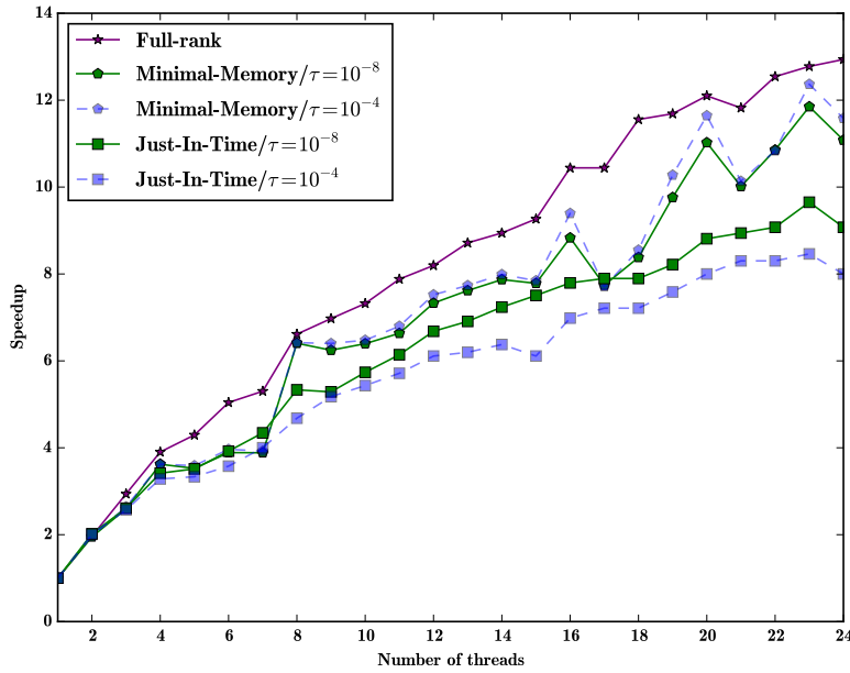
Figure 13: Speedup of the factorization for the atmosmodj matrix with 1 to 24 threads.
