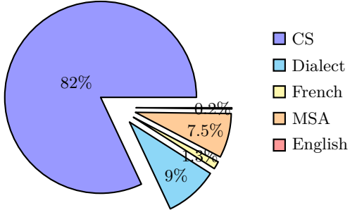
Figure 2: Code-switching distribution
