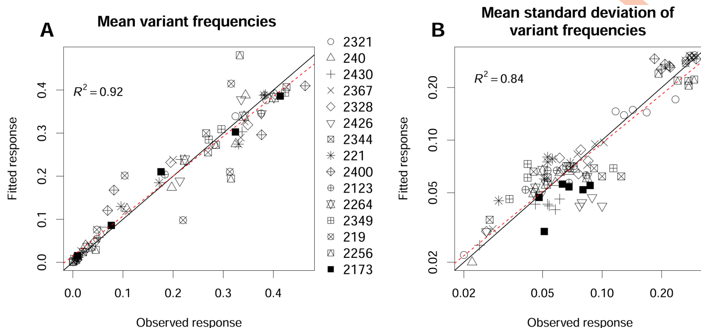
Fig 5. Goodness-of-fit of the Wright-Fisher model \mathcal{M}_4 with the data of the biological experiments. (A) Correlation between the observed mean frequencies of the five virus variants (averaged over all virus populations and sampling times ( \text{mean}[f_i^*(t_d)] )) and their fitted values ( n = 75 ). (B) Correlation between the logarithm of the observed mean (averaged over the variants) standard deviation of variant frequencies (between virus populations) at each sampling date t_d ( 1/n_{\text{var}} \sum_{i=1}^{n_{\text{var}}} \sigma[f_i^*(t_d)] ) and their fitted values ( n = 87 ). In both panels, the black line is the first bisector and the red dashed line is the best-fitting linear model.
