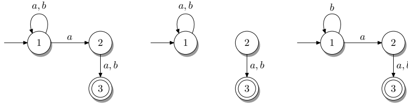
Fig. 1. Left: the NFA M with a sole nondeterministic state accepting the language (a+b)^*a(a+b) . Interpreting M as an OTNFA results in accepting b^*a(a+b) . Middle: partial DFA M' built from M by choosing the a -self-loop on the state 1 and deleting all other a -transitions leaving state 1. Right: partial DFA M'' built from M by choosing the a -transition from state 1 to 2 and deleting all other a -transitions from state 1.
