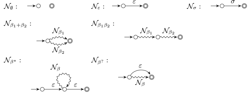
Fig. 1. The \varepsilon -follow construction, \mathcal{A}_{ef} .
