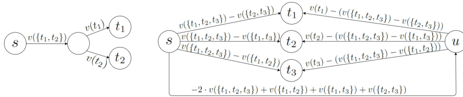
Fig. 2. Compressing flow networks with two and three sinks
