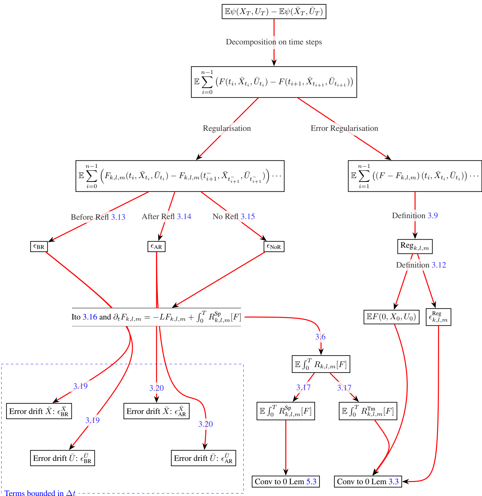
Figure 2: General Schematic of introduced definitions in the main Theorem 1.6
