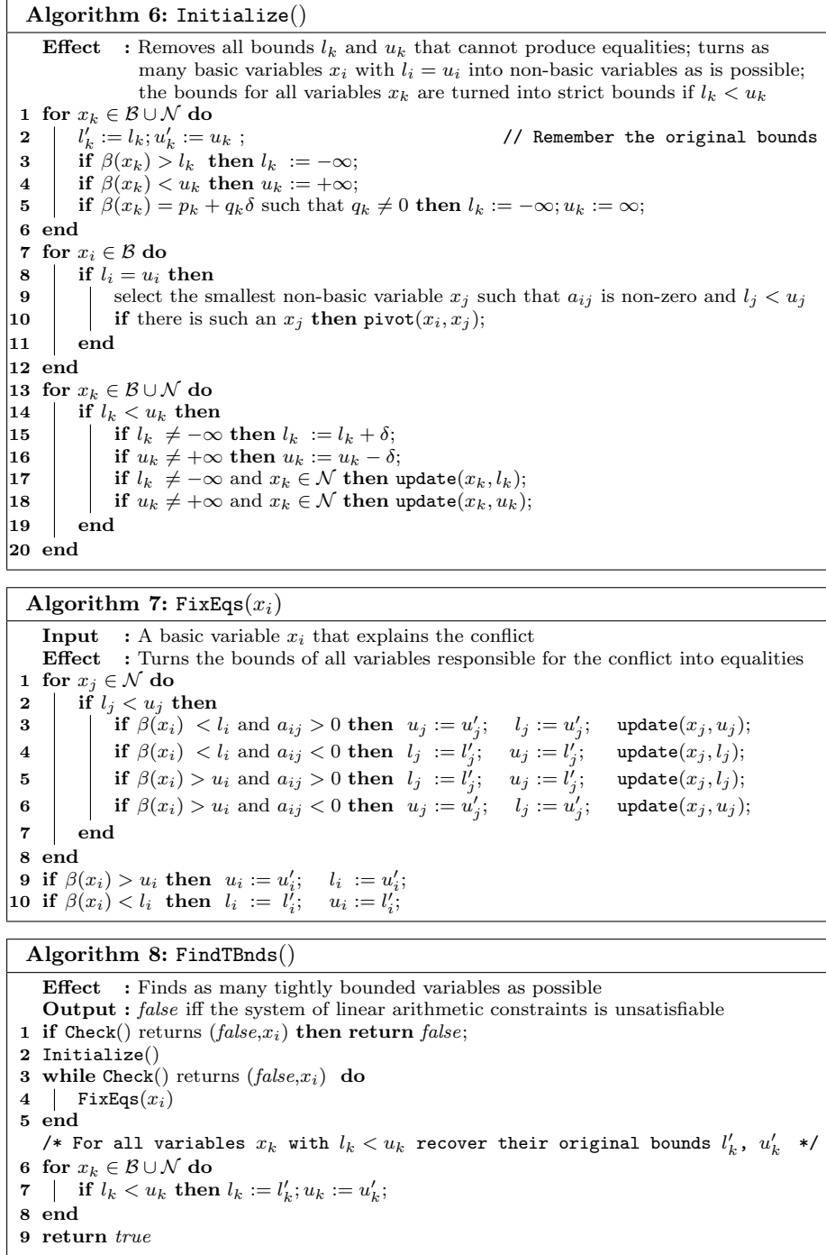
Fig. 6 The functions used to turn our original tableau into a basis of equalities
