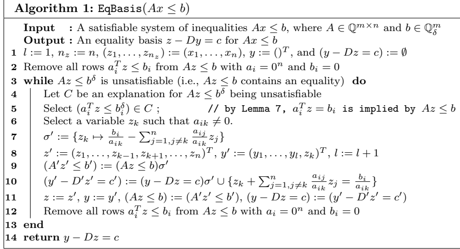
Fig. 4 EqBasis computes an equality basis
