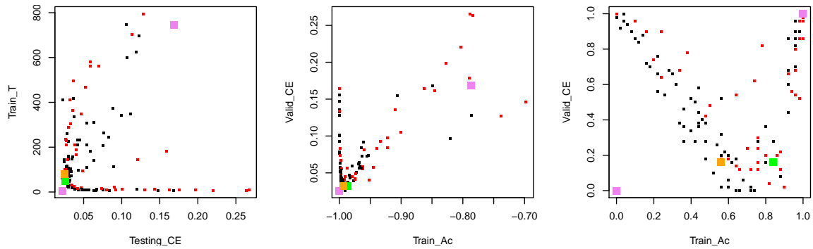
Figure 8: Projections on 2D spaces of the 150 observations, either in the original space (left, middle) or the copula space (right). The colors match the ones of Figure 7.
