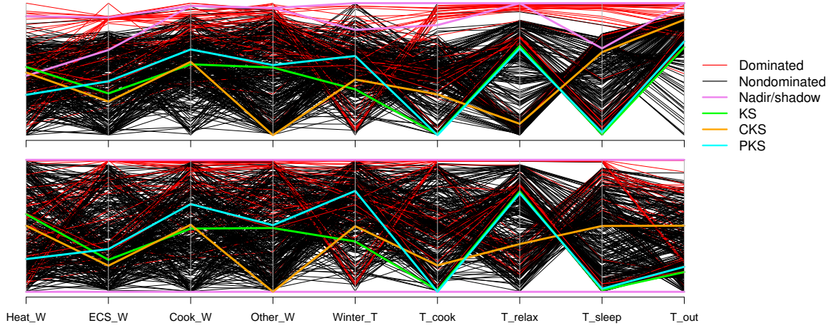
Figure 10: Parallel coordinates of the 400 observations, nadir and utopia points in the original (top) and copula (bottom) objective spaces (each line corresponds to a single observation, where objectives are rescaled on the graph). The colors highlight the dominated solutions and retained (KS, CKS and PKS) solutions.
