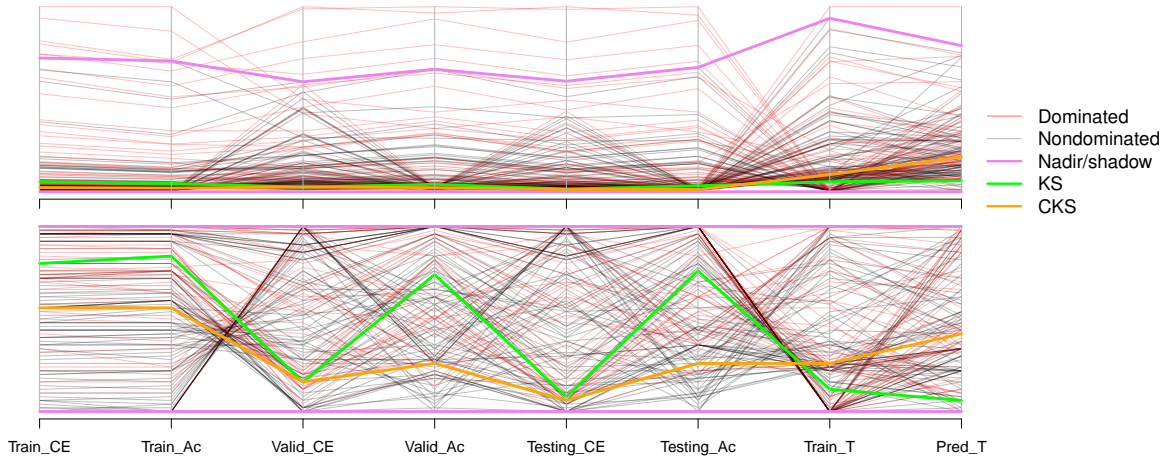
Figure 7: Parallel coordinates of the 150 observations, nadir and utopia points in the original (top) and copula (bottom) objective spaces (each line corresponds to a single observation, where objectives are rescaled on the graph). The colors highlight the dominated solutions and retained (KS and CKS) solutions.
