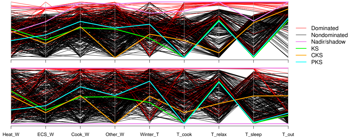
Figure 10: Parallel coordinates of the 400 observations, nadir and utopia points in the original (top) and copula (bottom) objective spaces (each line corresponds to a single observation, where objectives are rescaled on the graph). The colors highlight the dominated solutions and retained (KS, CKS and PKS) solutions.
