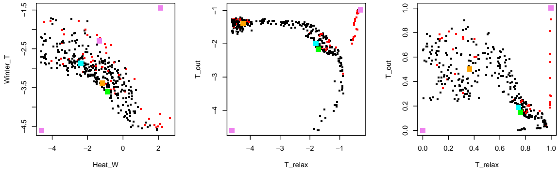
Figure 11: Projections on 2D spaces of the 400 observations, either in the original space (left, middle) or the copula space (right). The colors match the ones of Figure 10.
