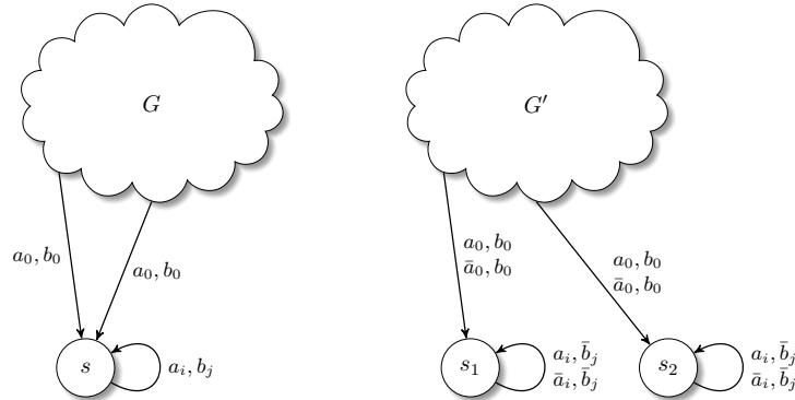
Fig. 3. How to make an automaton with sink state reversible. Automaton G is reversible except for the sink state s , where 0 \leq i, j \leq |B| - 1 (left). Automaton G' is reversible including the two sink states s_1 and s_2 (right). Every edge in G labeled a, b is labeled a, b and \bar{a}, b in G' which preserves weak reversibility.
