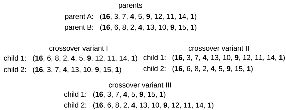
Fig. 1: Example of 2-point crossover. Given two parents which have 4 common vertices (16, 4, 9, 1) there are three possible fragment exchanges between successive points. Variant I shows children created by fragments exchange between vertices 16 and 4, variant II is created by segments exchange between points 4 and 9 while variant III shows offspring individuals created by exchange of fragments between vertices 9 and 1.
