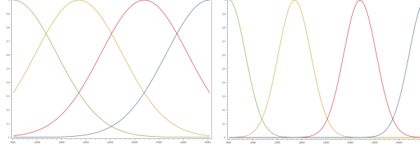
Fig. 2. Example division of decision attribute into four contexts using gaussian function with context configuration value (from left) 0.6 and 1.6.
