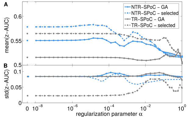
Figure 1. Sensitivity analysis wrt. the regularization strength for TR-SPoC and NTR-SPoC. (A) Averaged z -AUC performance is reported as grand average (GA) across all 18 subjects (solid line) and for five good subjects (dashed line). (B) Standard deviations of the corresponding averages are depicted. For comparison, the displayed performance at \alpha = 0 corresponds to the non-regularized SPoC versions.
