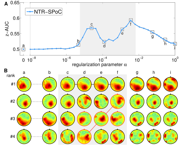
Figure 3. Effect of regularization parameter upon the performance and the spatial patterns for an exemplary subject VP9. (A) Performance of NTR-SPoC for choosing \alpha \in [10^{-8}, 10^0] . (B) Corresponding activity patterns along first four ranked components at the marked evaluation points (a)-(i).
