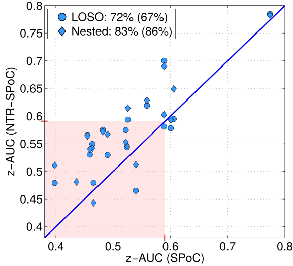
Figure 2. Performance comparison of NTR-SPoC with standard SPoC, using both LOSO and nested cross-validation. Each blue marker corresponds to one of the 18 subjects. For both of the selection strategies, the first number reports the percentage of subjects for which NTR-SPoC outperforms SPoC. Percentage values given in brackets are restricted to those data points located outside the red shaded area. It encloses all subjects which do not reach a threshold criterion on z\text{-AUC} for meaningful predictions.
