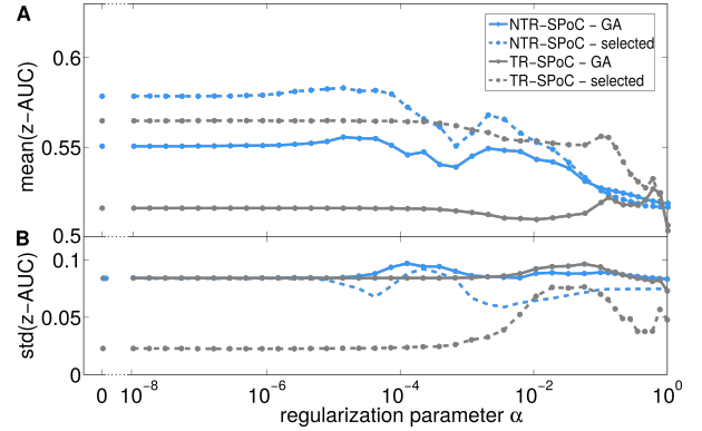
Figure 1. Sensitivity analysis wrt. the regularization strength for TR-SPoC and NTR-SPoC. (A) Averaged z -AUC performance is reported as grand average (GA) across all 18 subjects (solid line) and across a selected set of five subjects (dashed line) enclosing the 60-90th percentile wrt. z -AUC of SPoC. (B) Standard deviations of the corresponding averages are depicted. For comparison, the displayed performance at \alpha = 0 corresponds to the non-regularized SPoC versions.
