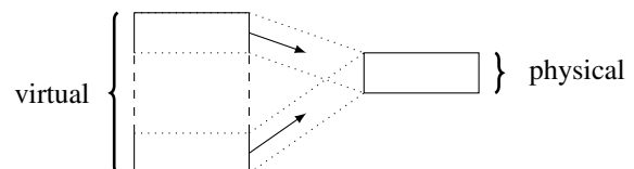
Figure 4. SMPI shared malloc mechanism: large area of virtual memory are cyclically mapped onto the same physical pages.
