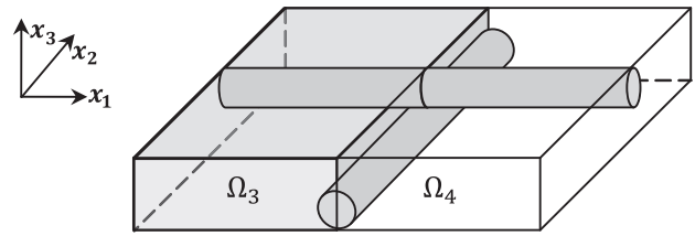
Fig. 2-3. Detail of the layer \Omega_3 \cup \Omega_4 including concrete and steel grid.
