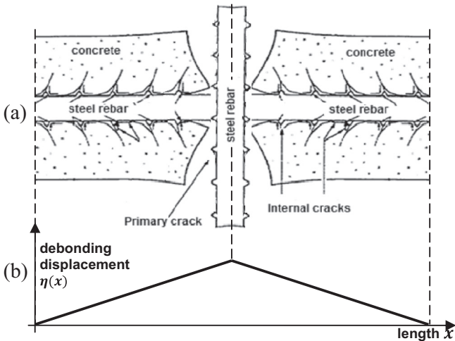
Fig. 2-1. (a) Debonding phenomena at concrete-steel rebar interface (Goto, 1971) (b) Assumed debonding displacement distribution at the interface.
