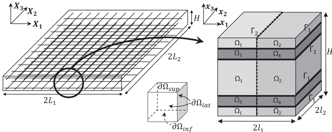
Fig. 2-2. Definition of the considered periodic cell from the real RC plate.
