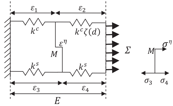
Fig. 3-2. Rheological model representing schematically the unit cell of Fig. 2-2 in one dimension.
