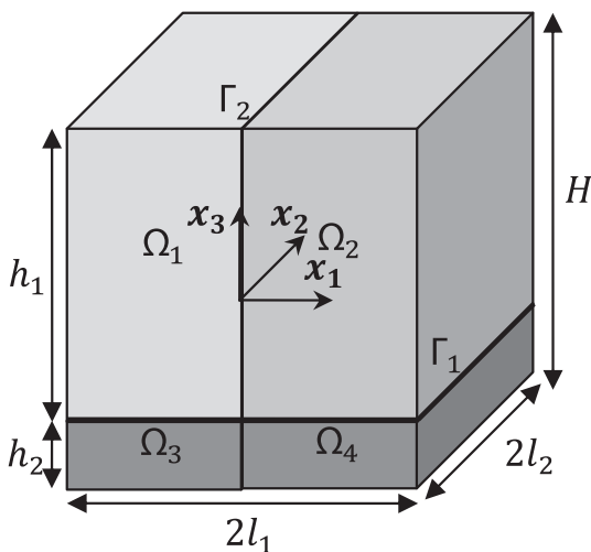
Fig. 3-1. Definition of the one dimensional periodic unit cell.
