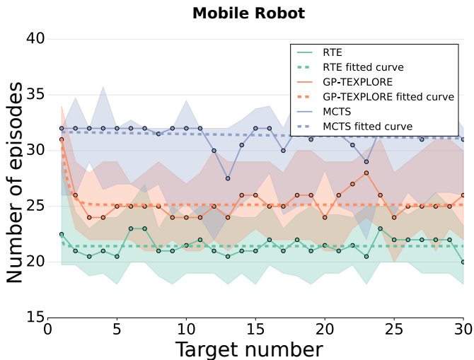
Figure 7: Median number of episodes to reach each target for a typical run of the algorithm for the mobile robot task. Over time, the robot using RTE or GP-TEXPLORE is able to reduce the number of required episodes to reach the next target (bottom lines), whereas MCTS alone uses a constant number of episodes (top line). Furthermore, RTE is able to correct its repertoire after the first target and outperforms GP-TEXPLORE, although the latter is capable of planning in the full action space. Most of the variance comes from the fact that the random targets are equidistant, but not of the same difficulty. The thick lines represent the medians over 50 runs and the shaded regions the 25 th and 75 th percentiles.
