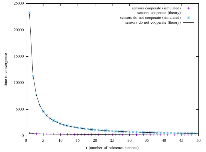
Figure 4. Time to converge (p = 10000, s = 150, \gamma = 0)
