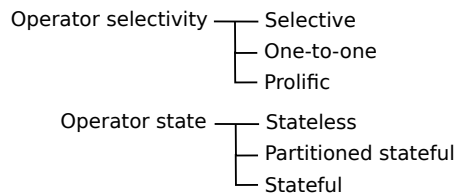
Figure 3: Types of operator selectivity and state.
