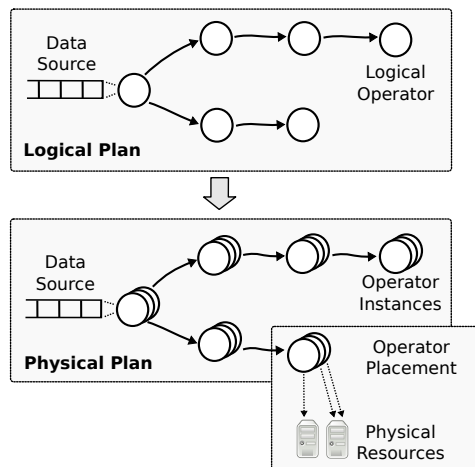
Figure 2: Logical and physical operator plans.
