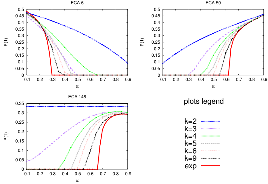
Figure 8: Local-structure approximations obtained for various approximation levels of order k (see Ref. [FF15] for details). For the sake of readability of the results, the cases k = 7 and k = 8 are omitted. The plot in red (label “exp”) shows the experimental steady-state density obtained for a ring size of n = 40\,000 cells after 10 000 time steps.
