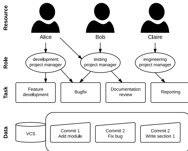
Fig. 7: Software project and resources
