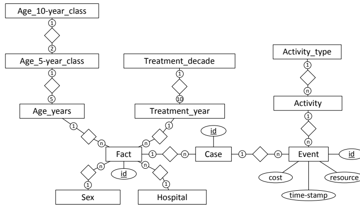
Fig. 8: Example database schema for the running example
