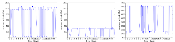
Fig. 2: Location time series for three distinct users during three weeks: humans tend to revisit locations in a periodic fashion. The visited locations are mapped to sequential identifiers, upon discretization on a regular grid of 50 meters step.
