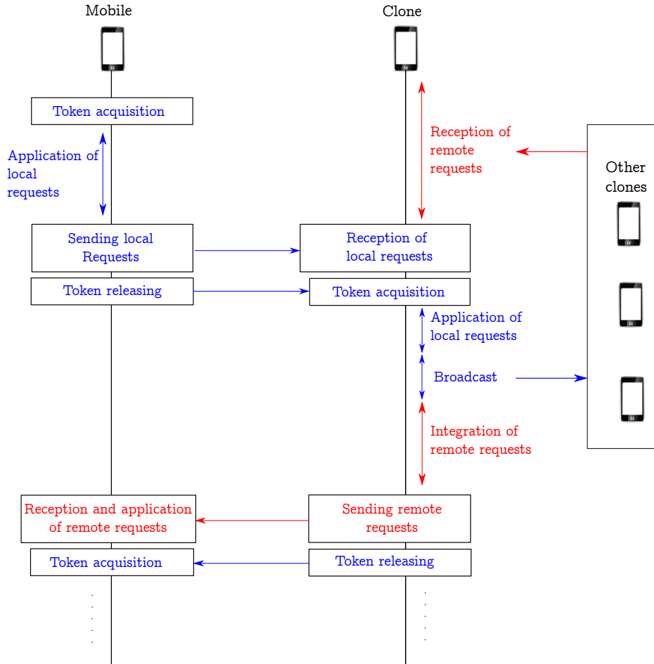
Figure 6 Consistency model.
