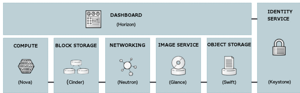
Figure 1: OpenStack Modules [4]
