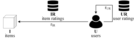
Fig. 3. Common feedback model of recommender and reputation systems.
