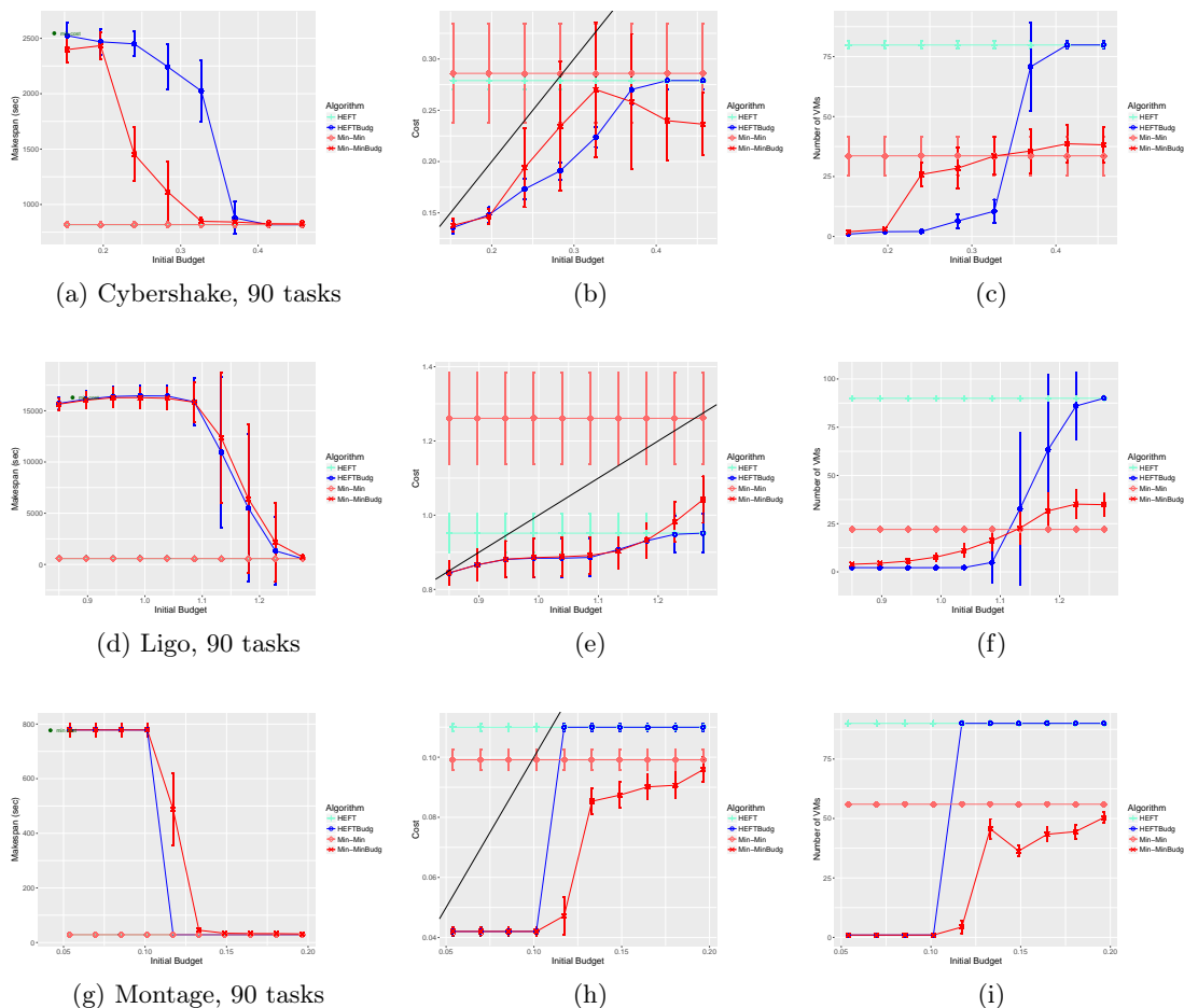
Figure 4: MIN-MIN, HEFT, budget-aware extensions MIN-MINBUDG and HEFTBUDG for the three workflow types with 90 tasks.
