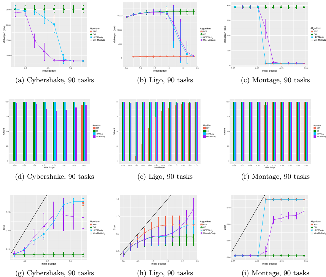
Figure 12: Makespan, percentage of valid schedules and cost for MIN-MINBUDG, HEFTBUDG, BDT and CG for CYBERSHAKE, LIGO and MONTAGE with 90 tasks.
