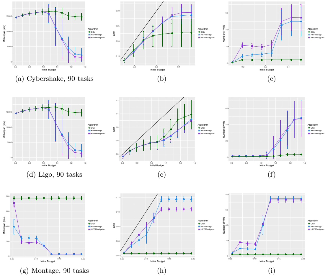
Figure 13: HEFTBUDG+ and HEFTBUDG+INV compared to CG+ for the three workflow types with 90 tasks.
